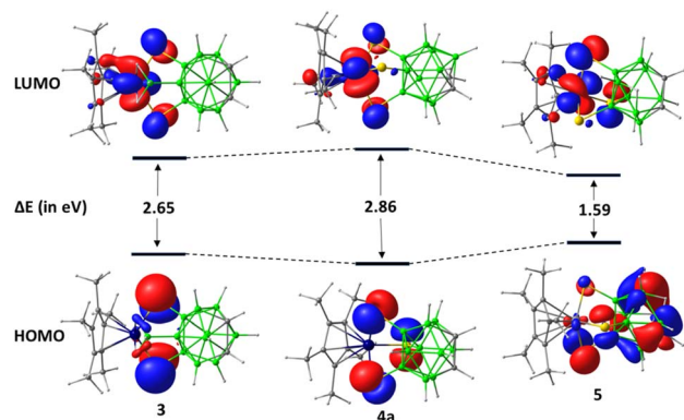
Fig. 9 Presentation of the energy levels, HOMO–LUMO gap, and orbital composition distribution of the HOMO and LUMO for 3 , 4a , and 5 (isocontour values: \pm 0.045 [e bohr ^{-3/2} ]).
