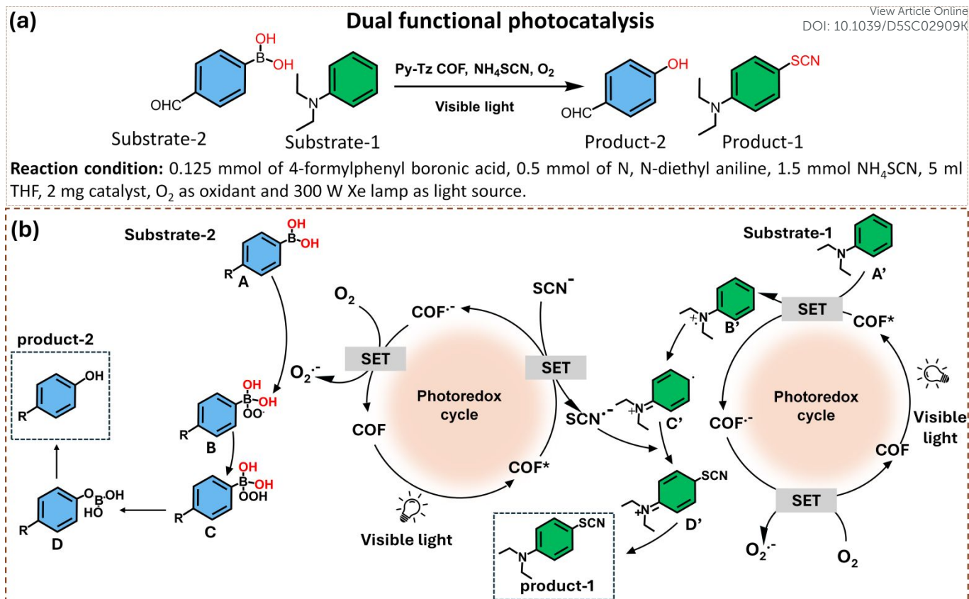
Figure 4. (a) Reaction condition and (b) plausible mechanism of dual-functional photocatalysis mediated by Py-Tz COF.
