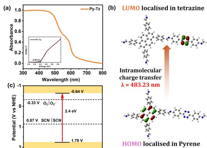
Figure 2. (a) Solid-state UV-Vis spectra and Tauc plot of Py-Tz COF (inset). (b) Electronic distribution of HOMU-LUMO of Py-Tz COF obtained from DFT calculation. (c) Schematic band diagram of Py-Tz COF indicating the valence band and conduction band position with respect to E_0 ( O_2|O_2^{\bullet-} ) and E_0 ( SCN^-|SCN^{\bullet-} ).
