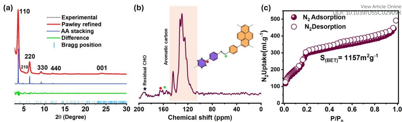
Figure 1. (a) PXRD patterns of Py-Tz COF; experimental obtained (dotted black), Pawley refined (red), simulated pattern for AA stacking (blue) and their difference (green). (b) Solid-state ^{13}\text{C} NMR spectra of Py-Tz COF. (c) \text{N}_2 adsorption isotherm of Py-Tz COF measured at 77K.
