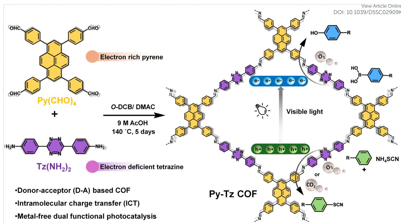
Scheme 1. Synthetic scheme of donor-acceptor Py-Tz COF from Py(CHO) 4 and Tz(NH 2 ) 2 , serving as a metal-free dual-functional heterogeneous photocatalyst. Two different organic transformation reactions: e^- -catalysed hydroxylation and h^+ -catalysed thiocyanation reactions conducted in a single pot.
