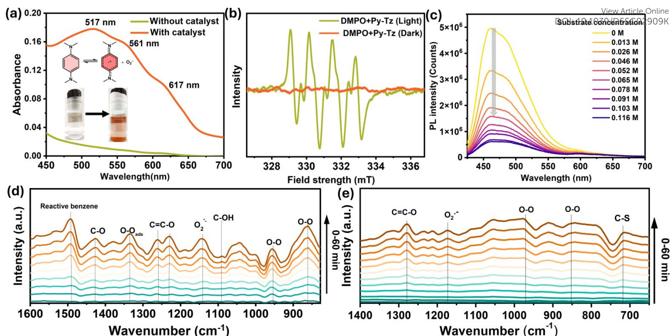
Figure 3. (a) UV-Vis spectra of TMPD radical cation formed by Py-Tz COF in the presence of light and O_2 . (b) EPR spectra of DMPO- O_2^- formed by Py-Tz COF in the presence of light. (c) Photoluminescence quenching experiment of Py-Tz COF in THF dispersion by varying concentrations of N,N-dimethylaniline. In-situ DRIFT studies demonstrate the appearance of new peaks, showing the progression of (d) hydroxylation reaction and (e) thiocyanation reaction.
