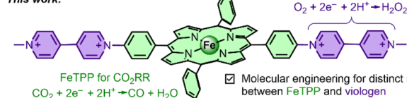
Scheme 1 Strategies for the electrocatalytic CO 2 RR in the presence of oxygen.
