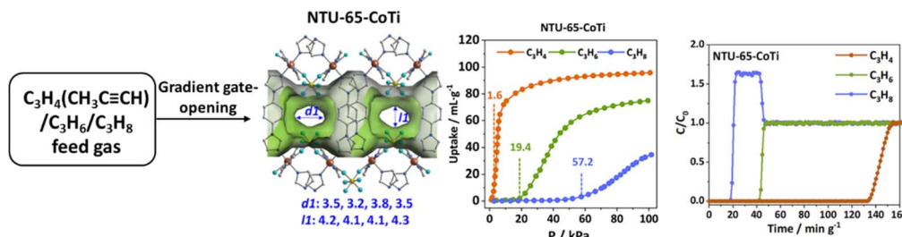
Fig. 19 The crystal structure of NTU-65-CoTi, adsorption isotherms for C_3H_4 , C_3H_6 and C_3H_8 at 273 K, and breakthrough experimental curves of C_3H_4/C_3H_8 (0.5/49.75/49.75, v/v/v, 2 mL min -1 ) mixtures at 273 K. Reprinted with permission from ref. 51. Copyright 2024 The Royal Society of Chemistry.
