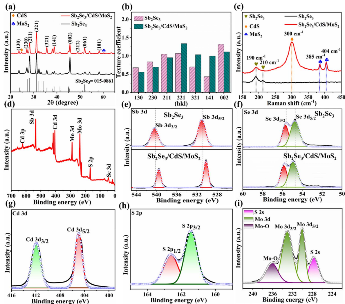
Fig. 2 (a) XRD, (b) texture coefficient of XRD peaks, and (c) Raman spectra of bare Sb 2 Se 3 and Sb 2 Se 3 /CdS/MoS 2 samples. (d) XPS survey graph of Sb 2 Se 3 /CdS/MoS 2 , the binding energy displacement of (e) Sb and (f) Se. XPS spectra for (g) Cd 3d, (h) S 2p, and (i) Mo 3d.
