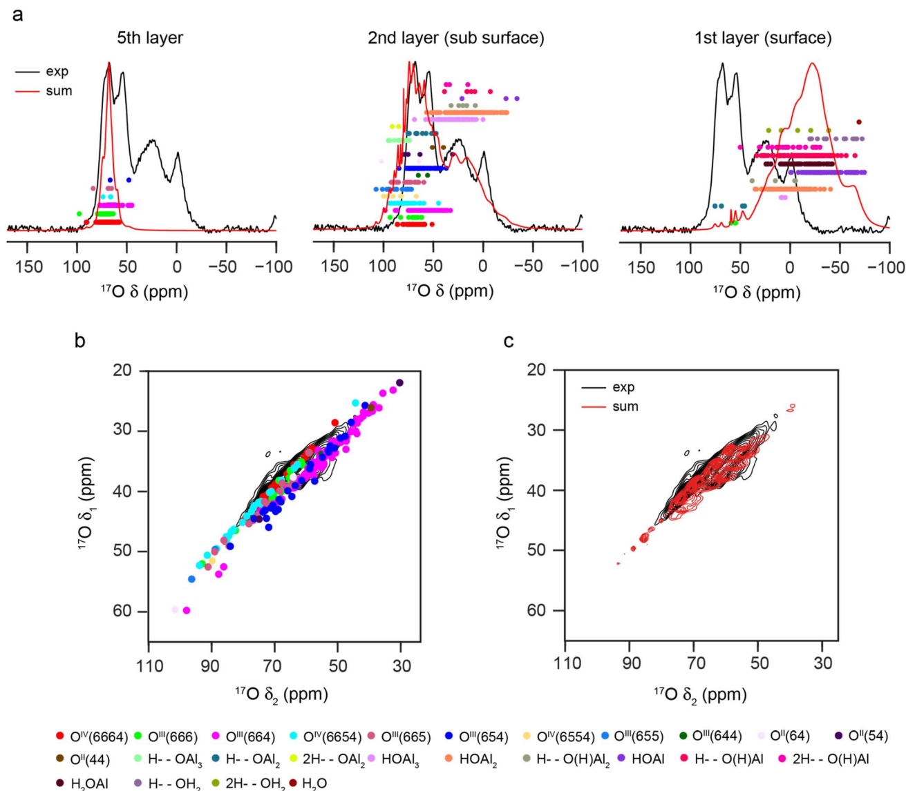
Fig. 6 (a) Plots showing the overlay of the DFT-predicted NMR shifts ( \delta_2 ) for all O in the slab models of \gamma -Al 2 O 3 , separated by the number of layers from the surface, with the ^{17}\text{O} (20.0 T, 20 kHz) MAS NMR spectrum of \gamma -Al 2 17 O 3 (500 °C) from Fig. 2a. The red line results from co-adding Lorentzian lineshapes simulated for each O species, centred at the \delta_2 centre-of-gravity with a FWHH proportional to C_Q . (b and c) Plots showing the overlay of ( \delta_1 , \delta_2 ) centre-of-gravity shifts predicted (using DFT) for non-protonated O environments in sub surface layer of the slab models of fully hydroxylated \gamma -Al 2 O 3 , with the ^{17}\text{O} (20.0 T, 30 kHz) DQF-STMAS spectrum of \gamma -Al 2 17 O 3 (950 °C) from Fig. 2b. In (c), the red contours represent the spectrum simulated from the sum of Lorentzians for each of the points in (b), with a FWHH of 1.5 ppm in \delta_1 and C_Q/\text{MHz ppm} in \delta_2 the ESI.†
