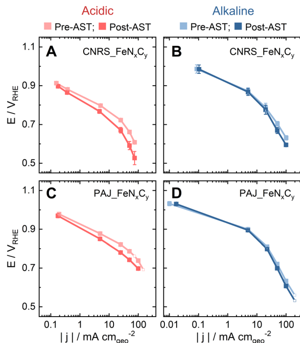
Fig. 1 Tafel plots of the pristine (pre-AST) and degraded (post-AST) Fe–N–C gas diffusion electrodes in \text{O}_2 at 70 \pm 6^\circ\text{C} in the gas diffusion electrode half-cell (A & B) using CNRS- \text{FeN}_x\text{C}_y as the catalyst (A) in 0.1 M \text{HClO}_4 and (B) in 0.1 M \text{NaOH} ; (C & D) using PAJ- \text{FeN}_x\text{C}_y as the catalyst (C) in 0.1 M \text{HClO}_4 and (D) in 0.1 M \text{NaOH} . The error bars represent the difference between the results of two experiments. The four blank square symbols show the data without repetition.
