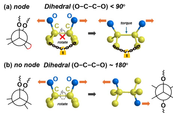
Fig. 2 Conformation of a “node” on the breaking C–C bond: (a) the dihedral angle of the designated C–C bond is less than 90° (i.e., with a node), inhibiting force transduction and generating torque on the bond. This results in severe distortion of bond angles and elongation of the bond length. (b) The dihedral angle is 180° (i.e., without a node), allowing force to pass freely. No significant distortion of bond angles or bond length is observed in this case.
