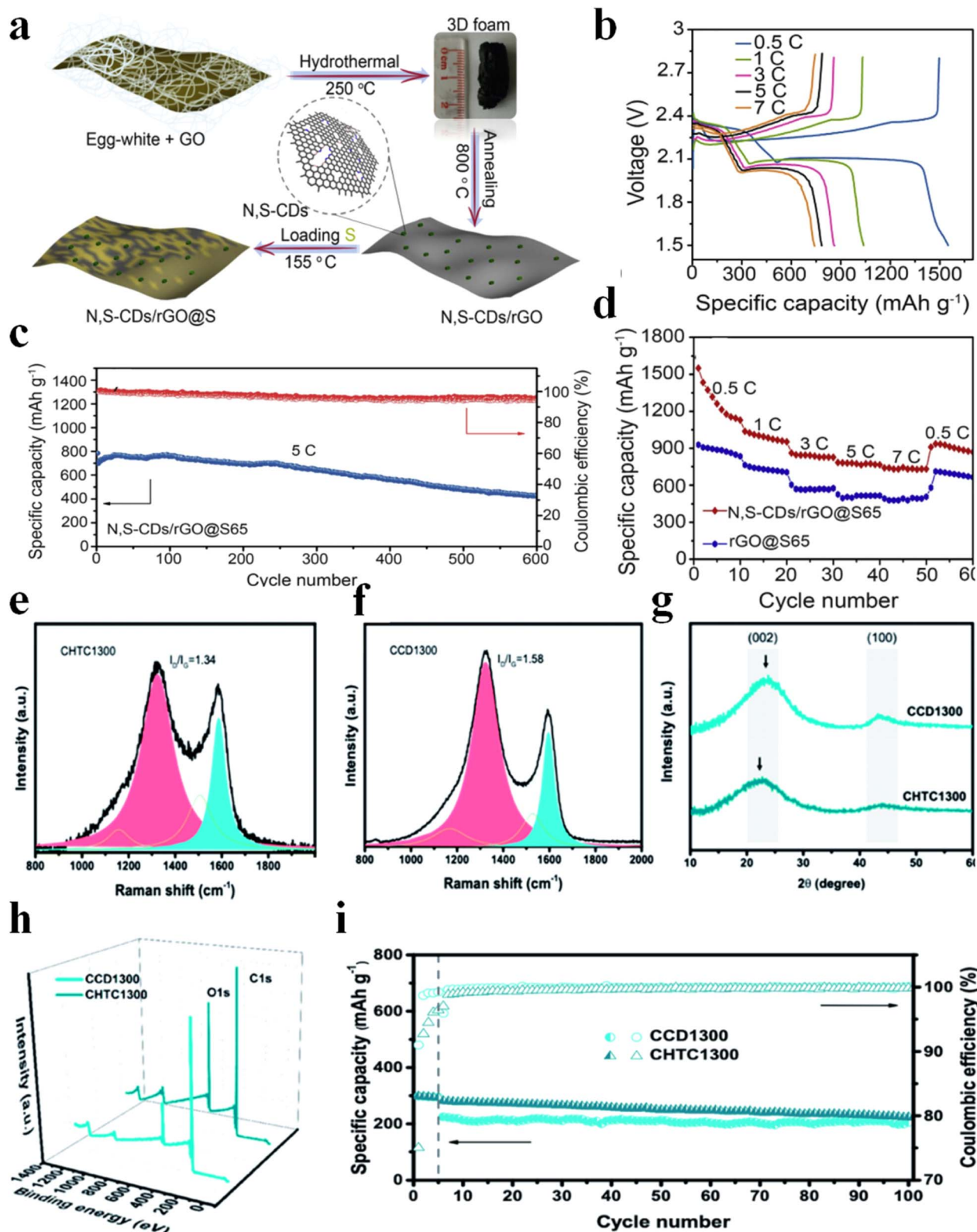
Fig. 7 CDs from egg white and cellulose: (a) a schematic diagram depicting the fabrication process of the N,S-CDs/rGO@s65 composites; (b) the charge/discharge profiles of N,S-CDs/rGO@s65 at various rates; (c) long-term cycling stability of N,S-CDs/rGO@s65 at 5C for 600 cycles; (d) rate performance comparison between N,S-CDs/rGO@s65 and rGO@s65; (a–d) reproduced with permission. 112 Copyright 2019, Elsevier. (e) Raman spectra of CHTC1300 and (f) CCD1300; (g) XRD patterns; (h) XPS survey; (i) cycling stability of CCD1300 and CHTC1300 in half cells at a current rate of 150 mA g -1 (with the initial five cycles conducted at 30 mA g -1 ). (e–i) Reproduced with permission. 113 Copyright 2019, Royal Society of Chemistry.
