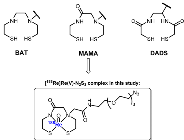
Fig. 1 Examples of N_2S_2 chelators for chelating ^{99m}\text{Tc}(\text{v}) and ^{186/188}\text{Re}(\text{v}) , and the [ ^{188}\text{Re} ]Re(v)- N_2S_2 complex used in this study.
