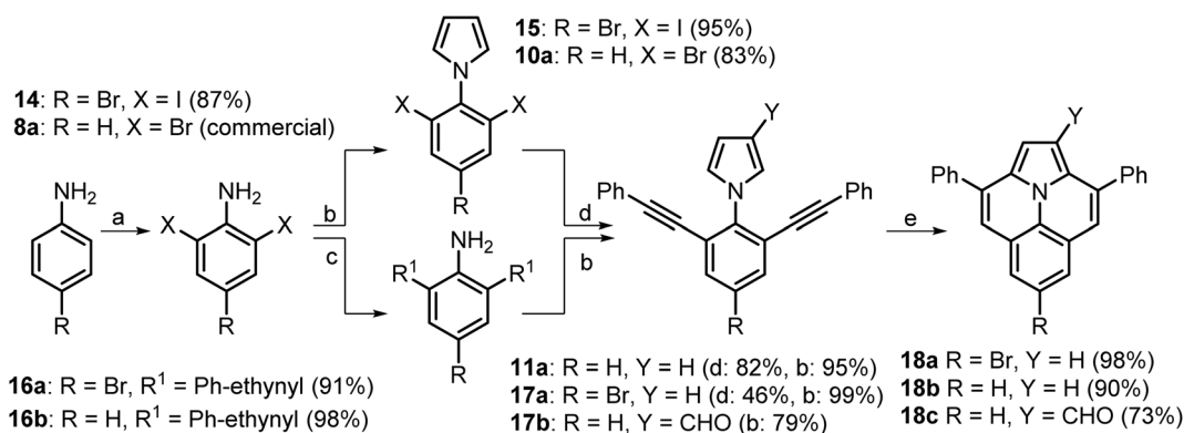
Scheme 3 Synthesis of ullazines 18a–c . Conditions: (a) ICl, MeOH, reflux (for 14a ); (b) Claisen–Kaa reaction: 2,5-dimethoxytetrahydrofuran (for 15a , 15b , 17a , 17b ) or 2,5-dimethoxy-3-tetrahydrofurancarboxaldehyde (for 12c ), AcOH, DCE, reflux; (c) PhCCH, CuI, Pd(PPh 3 ) 4 , Et 3 N, THF, r.t. (for 16a ) or Et 3 N-neat, 90 °C (for 16b ); (d) PhCCH, Pd(CH 3 CN) 2 Cl 2 , XPhos, Cs 2 CO 3 , CH 3 CN, 60 °C (for 17a ); PhCCH, Pd(CH 3 CN) 2 Cl 2 , tBu 3 P, Cul, diisopropylamine, 1,4-dioxane, r.t. (for 17b ); (e) InCl 3 , toluene (for 18a , 18c ) or o-xylene (for 18c ), reflux.
