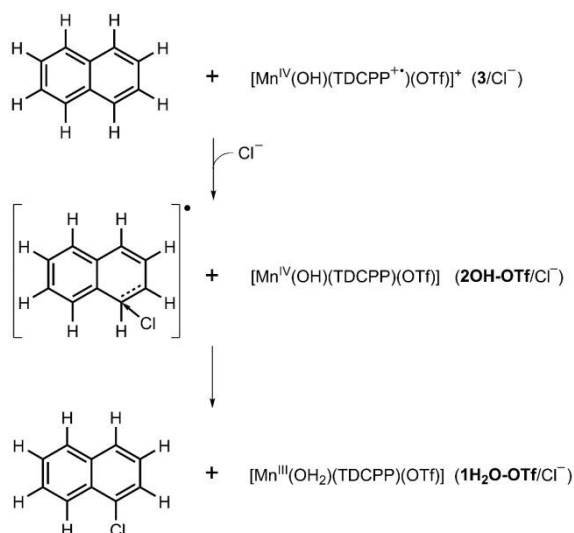
Scheme 2 Proposed halogenation pathway of naphthalene substrate. At the intermediate stage in this reaction, the Mn catalyst abstracts approximately half an electron from the substrate and the other half from the chloride.
