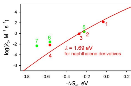
Fig. 4 Plot of \log k_2 for the oxidation of different substrates [(1) 1-Me-naphthalene, (2) naphthalene, (3) 1-Br-naphthalene; (4) 1-NO 2 -naphthalene; (5) anisole; (6) toluene; (7) benzene] vs. the driving force of electron transfer [ -\Delta G_{\text{et}} ; eqn (2)] by 3 /Cl − in CH 2 Cl 2 at -10^\circ\text{C} .
