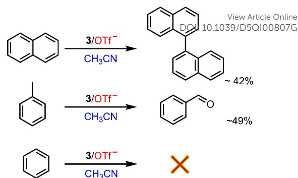
Fig. 2 Products with yield in the reaction of 3/OTf - (1.0 mM) with naphthalene (10 mM), toluene (200 mM), and benzene (400 mM) in CH 3 CN at -10 °C. 3/OTf - was generated by using [Mn III (TDCPP)(OTf)] (1.0 mM) with PhIO (5 equiv.) and HOTf (10 equiv.) at -10 °C.
