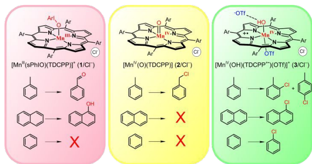
Scheme 1 Reactions of Mn-porphyrin intermediates with aromatic compounds.
