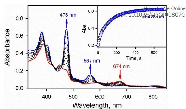
Fig. 1 UV-vis spectral change observed in the reaction of 3/Cl – (0.10 mM, red line) and toluene (0.40 M) in CH 2 Cl 2 /CH 3 CN (v/v 20:1) at –10 °C. Inset shows the time trace monitored at 478 nm. 3/Cl – (0.10 mM, red line) was generated in situ by the reaction of [Mn III (TDCPP)(Cl)] with PhIO (5 equiv.) and HOTf (10 equiv.).
