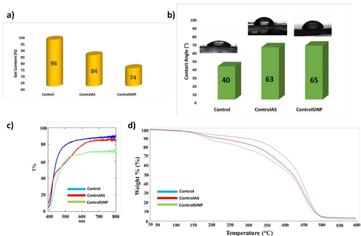
Fig. 18 The gel content values (a), water contact angle values (b), transmission spectra (c), and TGA thermograms (d) of the photosests.
