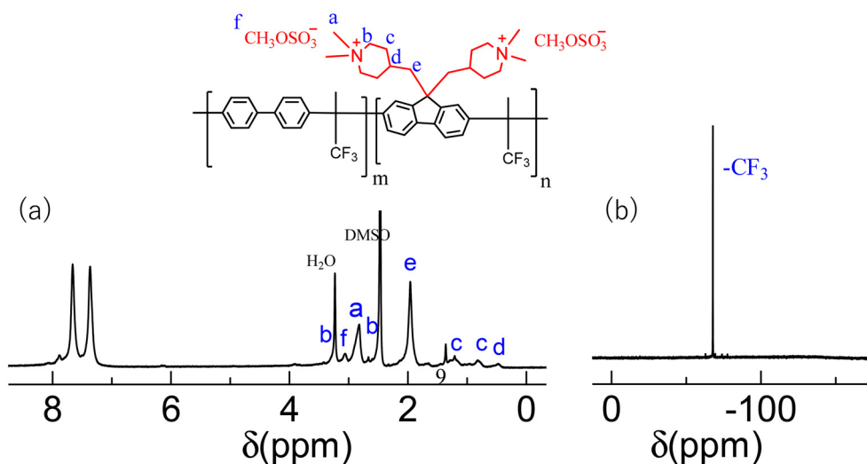
Fig. 1 (a) ^1\text{H} and (b) ^{19}\text{F} NMR spectra of quaternized QBPh-Pip copolymer.
