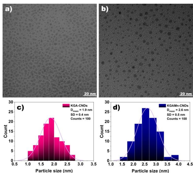
Figure 5. TEM images of KGA-CNDs (a), KGAMn-CNDs (b) with corresponding particle size distribution histograms: KGA-CNDs (c), KGAMn-CNDs (d).
