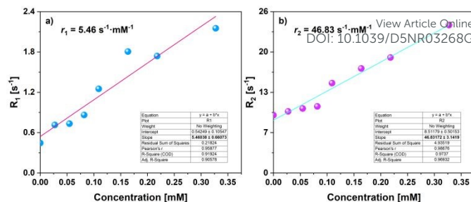
Figure 18. Linear fitting of R_1 (a) and R_2 (b) as a function of molar concentration of Mn comprised in KGAMn-CND. The slopes of the lines represent the relaxivities r_1 and r_2 , of 5.46 and 46.83 s^{-1} \cdot mM^{-1} , respectively.
