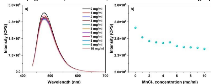
Figure 10. PL spectra of KGA-CNDs (a) and the variation of PL intensity (b) at the excitation wavelength of 420 nm as a function of MnCl_2 concentration.
