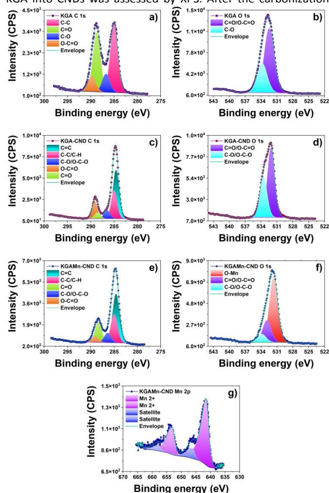
Figure 3. High-resolution XPS spectra of pure KGA: (a) C 1s and (b) O 1s; KGA-CNDs: (c) C 1s and (d) O 1s; and KGAMn-CNDs: (e) C 1s, (f) O 1s, (g) Mn^{2+} 2p.
