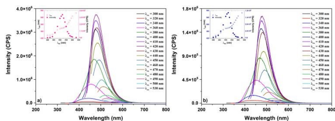
Figure 9. Photoluminescence emission spectra of KGA-CNDs (a) and KGAMn-CNDs (b) recorded at different excitation wavelengths. Insets: correlation between emission wavelength ( \lambda_{em} ), excitation wavelength ( \lambda_{ex} ), and PL intensity.
