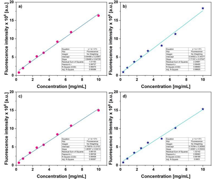
Figure 16. Graphs of linear dependence of fluorescence intensity on concentration of compounds KGA-CNDs (a,c) and KGAMn-CNDs (b,d). The upper line in the figure presents the graphs of the two compounds at the first scan (a,b), and the bottom line presents the graphs obtained after the 10th scan (c,d). The slopes of the lines slightly decrease from 1.59 and 1.71 to 1.46 and 1.44 for KGA-CND and KGAMn-CND, respectively.
