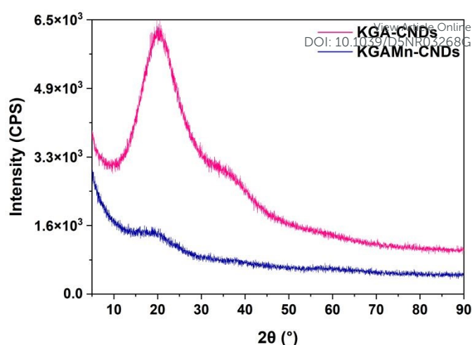
Figure 6. The diffractogram of KGA-CNDs (pink) and KGAMn-CNDs (blue).
