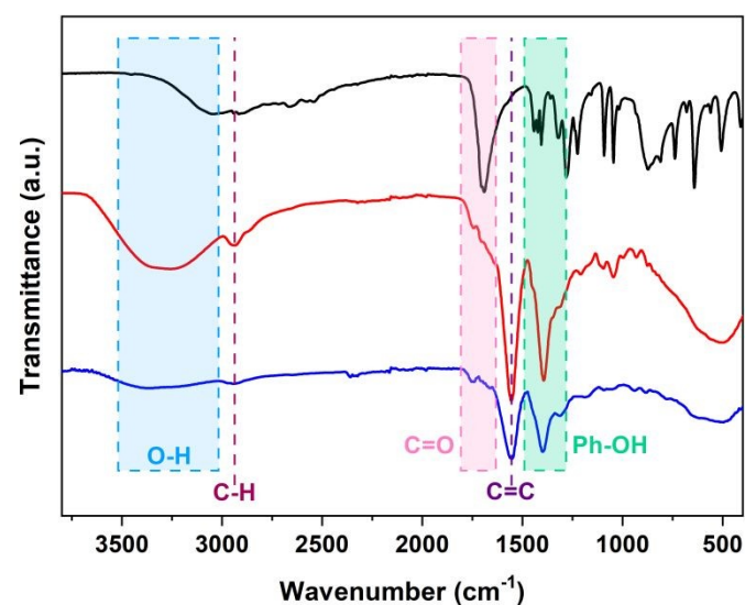
Figure 2. ATR FT-IR spectra of pure KGA (black), KGA-CNDs (red) and KGAMn-CNDs (blue).
