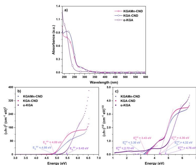
Figure 8. UV-Vis absorption spectra (a) of pure KGA, KGA-CNDs and KGAMn-CNDs. Direct (b) and indirect (c) allowed transitions calculated from the UV-Vis data.
