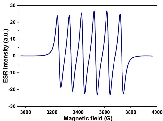
Figure 7. ESR spectrum of KGAMn-CNDs (10 mg/mL) in water, recorded at room temperature.
