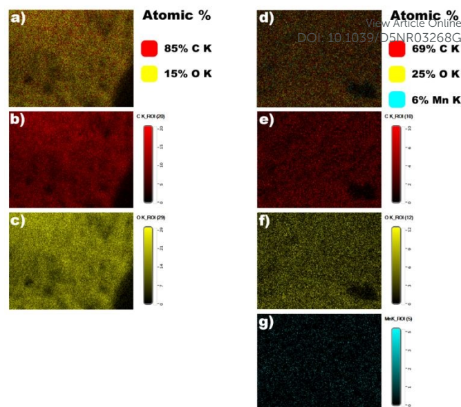
Figure 4. EDX elemental mapping of KGA-CNDs (a) and KGAMn-CNDs (d), illustrating the spatial distribution of carbon and oxygen in KGA-CNDs (b, c) and KGAMn-CNDs (e, f), as well as the presence of manganese in KGAMn-CNDs (g).
