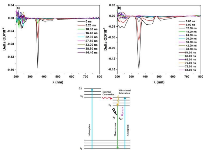
Figure 14. Transitions absorption spectra of KGA-CNDs (a) and KGAMn-CNDs (b) in water, along with an illustration of the energy diagram (c).
