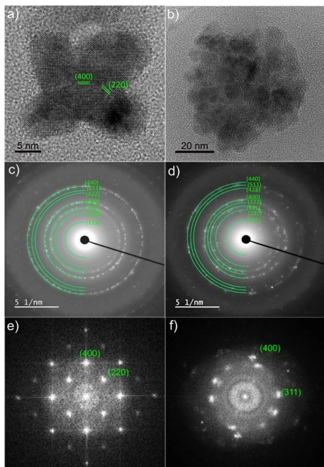
Figure 2. High-resolution TEM images of (a) 25 nm octopod-shaped Mn-Fe oxide NPs and (b) 50 nm Fe core-Mn shell NPs and their corresponding (c-d) SAED and (e-f) FFT analyses.
