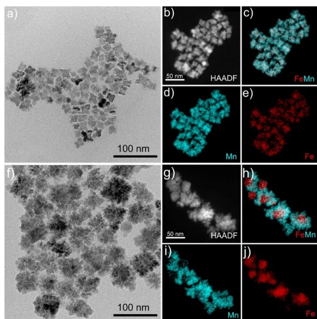
Figure 1. (a) TEM image of 25 nm octopod-shaped Mn-Fe oxide NPs synthesized after 15 min reaction time, (b) HAADF-STEM image, and (c–e) STEM-EDX maps of Mn/Fe, Mn and Fe. (f) TEM image of 50 nm Fe core-Mn shell NPs formed after a 60-min reaction time, (g) HAADF-STEM image, and (h–j) STEM-EDX maps of Mn/Fe, Mn and Fe.
