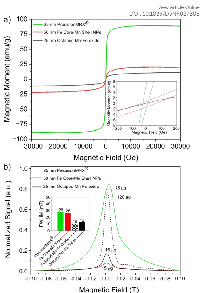
Figure 3. (a) The field-dependent magnetization curves and (b) the corresponding normalized PSF for 25 nm octopod-shaped Mn-Fe oxide NPs, 50 nm Fe core-Mn shell NPs, and 25 nm commercial PrecisionMRX ® iron oxide NPs. Relaxometry measurements were conducted at a sample concentration of 15 \mu\text{g} of total Fe and Mn per 1 mL solvent, except for the hatched graph, which represents signal data for 25 nm octopod Mn-Fe oxide NPs at a concentration of 120 \mu\text{g} of total Fe and Mn per 1 mL solvent.
