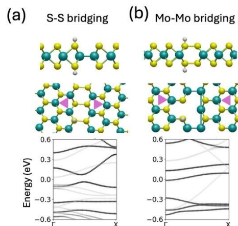
Figure 7: Fully relaxed atomic configuration of GBs with hydrogenation at the position of point defects. Two metallic types of GBs are investigated: (a) S-S bridging GB with single sulphur vacancy, (b) Mo-Mo bridging GB with single Mo vacancy. The Fermi-levels are aligned to 0 in all band structure plots. The side view and top view are provided for clear observation of the positions of the hydrogen atoms
