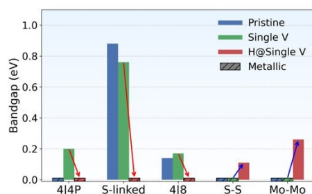
Figure 8: Bandgaps of various grain boundaries under three structural conditions—defect-free, single-defected and hydrogenated — plotted from left to right for each GB. Red arrows show the restoration of metallicity by hydrogenation, while the blue arrows show bandgap opening by hydrogenation.
