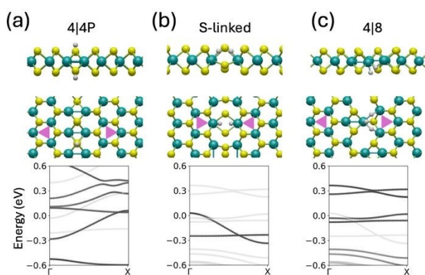
Figure 6: Fully relaxed atomic configuration of GBs with hydrogenation at the position of point defects. Three semiconducting types of GBs are investigated: (a) 4|4P, (b) S-linked GB and (c) 4|8 with single sulphur vacancies. The Fermi-levels are aligned to 0 in all band structure plots. The side view and top view are provided for clear observation of the positions of the hydrogen atoms
