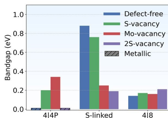
Figure 3: Bandgaps of representative mirror twin grain boundaries (4|4P, S-linked, and 4|8) under different defect conditions—defect-free, single sulphur vacancy, single molybdenum vacancy, and double sulphur vacancy—plotted from left to right for each GB.
