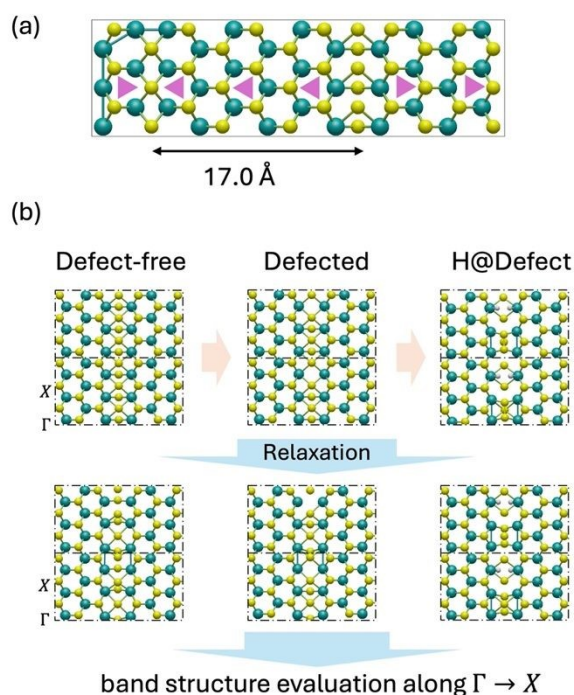
Figure 1: (a) Top view of the integral supercell containing two mirror-symmetric grain boundaries in parallel separated by 17 Å. The total size of the simulation cell is 33.4 \times 9.4 \times 18 \text{ Å}^3 . (b) Simulation workflow for studying the effects of defects and hydrogenation on grain boundaries (GBs) in monolayer \text{MoS}_2 , where S-linked GB is used here as an example. An ideal GB structure is first constructed and relaxed, and its electronic properties are assessed (first column). Point defects are then introduced, and the resulting structures are optimized and analysed (second column). Finally, hydrogen atoms are added at defect sites, and the passivated systems are further optimized to evaluate the impact on electronic behaviour (third column).
