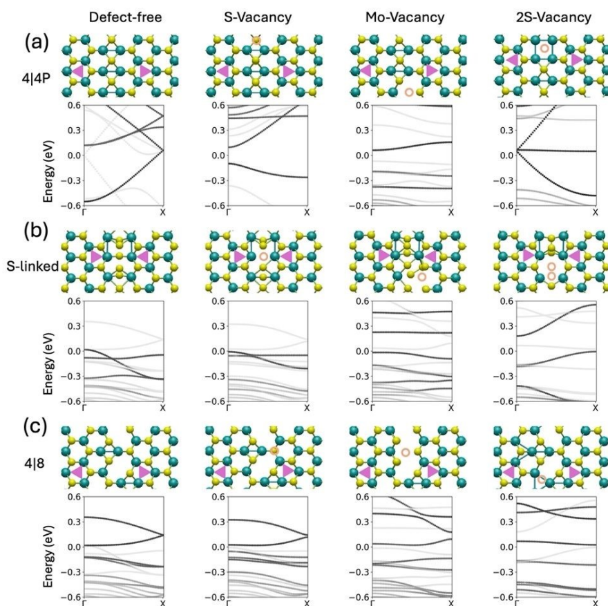
Figure 2: Atomic configurations and band structures for three representative GBs: (a) 4|4P, (b) S-linked GB and (c) 4|8, under different defect configurations. Each column corresponds to one type of defects: defect-free, S vacancy, Mo vacancy, and double sulphur vacancy (2S-vacancy) at the GB centre. The \Gamma -X path is plotted for all the cases. The orange circle is plotted for eye-guide at the position of defects and the triangles emphasize the orientation of the bulk domains. The atomic configurations are full relaxed. The Fermi levels are shifted to 0 in the band structure plots.
