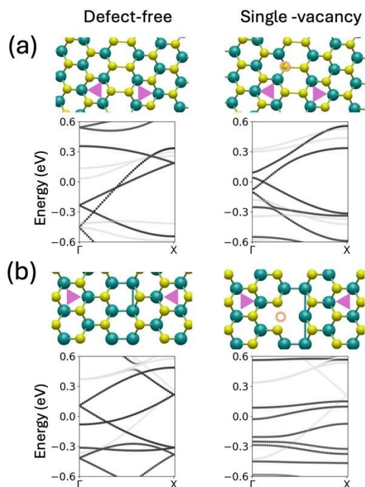
Figure 4: Fully relaxed atomic configurations of (a) S-S bridging and (b) Mo-Mo bridging GB, under defect-free structure (left column) and structure with single defects (right column). Single sulphur vacancy is introduced for S-S bridging GB while single Mo vacancy is introduced for Mo-Mo bridging GB. The orange circle is plotted for eye-guide at the position of defects and the triangles represent the orientation of the bulk domains. The Fermi levels are aligned to 0 in all band structure plots.
