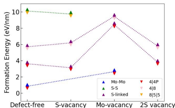
Figure 5: Formation energies of different grain boundaries and their defected forms, with formation energy of two GBs evaluated simultaneously within each unit cell.
