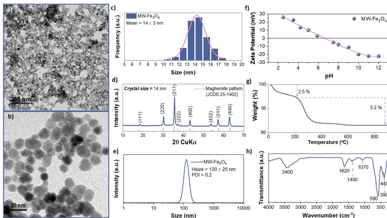
Fig. 1 Structural, compositional and colloidal characterization of the first batch of MW-Fe 3 O 4 (batch 2–8 characterization is shown in the ESI†). (a) and (b) TEM images, (c) particle size distribution, (d) X-ray diffraction pattern, (e) hydrodynamic size in intensity, (f) zeta potential (the solid line is a guide to the eye), (g) thermal gravimetric analysis and (h) infrared spectra.
