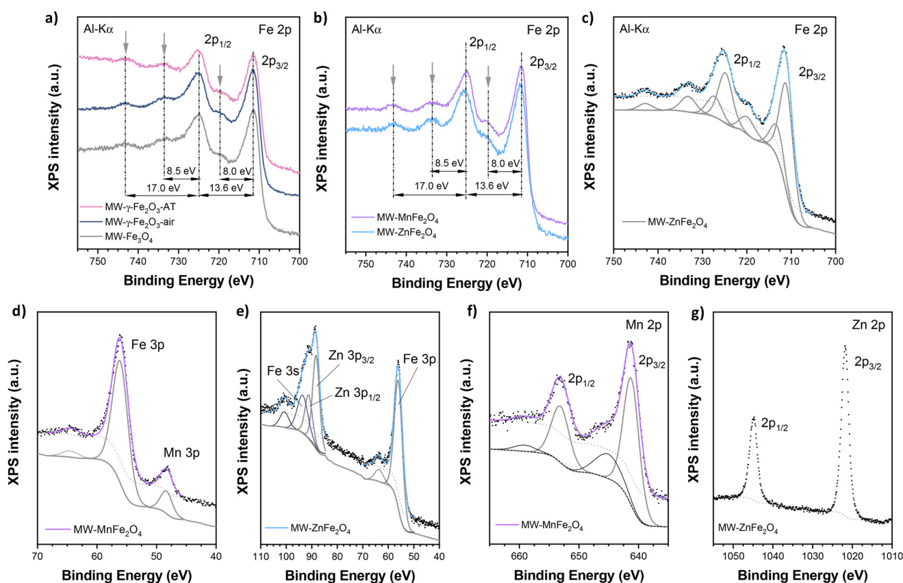
Fig. 7 Surface analysis by XPS. (a) XPS spectra of Fe 2p corresponding to the MW-Fe_3O_4 , MW-\gamma-Fe_2O_3 -air, MW-\gamma-Fe_2O_3 -AT samples. The XPS spectra were normalized to maximum peak intensity for better visual inspection and direct comparison between the samples. (b) Normalized XPS spectra of Fe 2p corresponding to the MW-Mn_{0.4}Fe_{2.6}O_4 and MW-Zn_{0.7}Fe_{2.3}O_4 samples. (c) XPS spectrum of Fe 2p corresponding to the MW-Zn_{0.7}Fe_{2.3}O_4 sample. Data points are represented as black solid symbols, Shirley background as dotted lines and components using solid lines, and the fitting curve as a light blue line. (d) Mn and Fe 3p spectra corresponding to the MW-Mn_{0.4}Fe_{2.6}O_4 sample. (e) Zn and Fe 3p spectra corresponding to the MW-Zn_{0.7}Fe_{2.3}O_4 sample. (f) Mn 2p spectra corresponding to the MW-Mn_{0.4}Fe_{2.6}O_4 sample. (g) Zn 2p spectra corresponding to the MW-Zn_{0.7}Fe_{2.3}O_4 sample.
