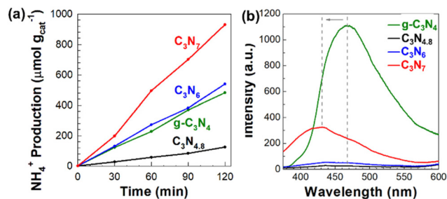
Fig. 6 (a) Amount of generated ammonia under a \text{N}_2 atmosphere and (b) PL spectra for exfoliated \text{g-C}_3\text{N}_4 , \text{C}_3\text{N}_{4.8} , \text{C}_3\text{N}_6 and \text{C}_3\text{N}_7 nanosheets.
