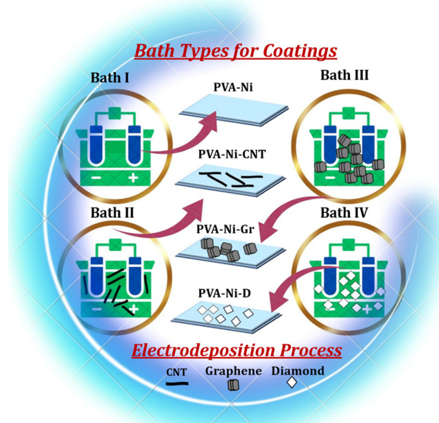
Fig. 1 Schematic representation of the bath types used in the electrodeposition process of the PVA-Ni, PVA-Ni-CNT, PVA-Ni-Gr and PVA-Ni-D composite coatings.
