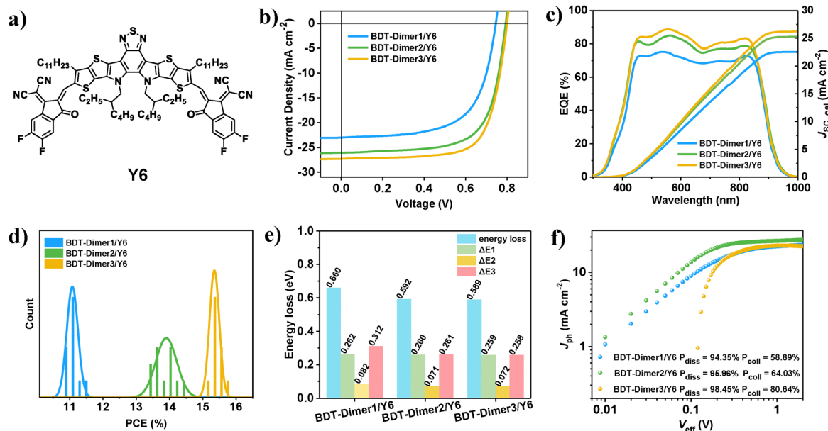
Fig. 4 Device performances. (a) Chemical structure of Y6, (b) optimized J-V curves, (c) corresponding EQE curves and (d) statistical distribution of optimized PCE, (e) energy loss and (f) V_{\text{eff}}-J_{\text{ph}} curves for optimized devices.
