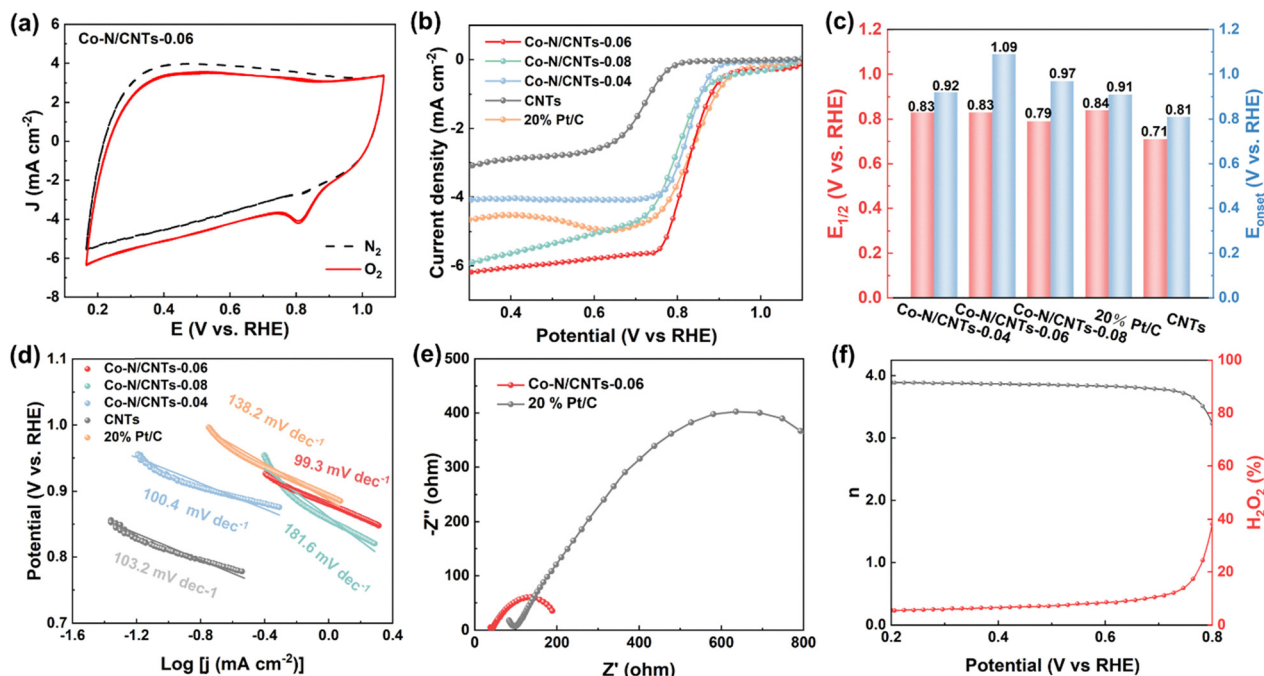
Fig. 3 (a) CV curves of Co-N/CNTs-0.06 in \text{N}_2 - and \text{O}_2 -saturated 0.1 M KOH at the scan rate of 10 \text{ mV s}^{-1} . (b) The linear sweep voltammetry (LSV) curves, (c) the half-wave potential and onset potential, and (d) Tafel plots of the ORR on CNTs, Co-N/CNTs-0.04, Co-N/CNTs-0.06, Co-N/CNTs-0.08, and 20% Pt/C in 0.1 M KOH solution at 1600 rpm. (e) EIS pattern of Co-N/CNTs-0.06 and 20% Pt/C recorded at 1.03 V vs. RHE. (f) Calculated n and determined \text{H}_2\text{O}_2\% at various potentials based on the RRDE.
