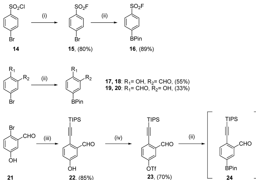
Scheme 1 Synthesis of aryl warheads as boronic esters. (i) KHF_2 , H_2O , MeCN, rt, 24 h; (ii) bis(pinacolato)diboron, KOAc, Pd(dppf)Cl_2 \cdot CH_2Cl_2 (10 mol%), 1,4-dioxane, 80 °C, 18 h; (iii) Pd(dppf)Cl_2 \cdot CH_2Cl_2 , CuI, triisopropylsilylacetylene, NEt_3 , 50 °C, 3 h; (iv) trifluoromethanesulfonyl chloride, NEt_3 , CH_2Cl_2 , 0 °C – rt, 2 h.
