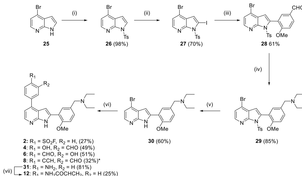
Scheme 2 Synthesis of compounds 2 , 4 , 6 and 8 . (i) TsCl , NaH, THF, 0 °C, 2 h; (ii) LDA, I_2 , THF, –78 °C, 3 h; (iii) (5-formyl-2-methoxyphenyl) boronic acid, Pd(PPh_3)_4 (10 mol%), Na_2CO_3 , 1,4-dioxane, \Delta , 12 h; (iv) diethylamine, NaBH(AcO)_3 , 1,4-dioxane, rt, 12 h; (v) CH_3OH , KOH, \Delta , 18 h; (vi) boronic ester, Pd(dppf)Cl_2 \cdot CH_2Cl_2 (5 mol%), Na_2CO_3 , 1,4-dioxane, \Delta , 0.5 h, \mu W ; (vii) acryloyl chloride, DIPEA, DMF, rt, 2 h. *Obtained using conditions (vi) followed by treatment with CsF in DMF, rt, 0.5 h.
