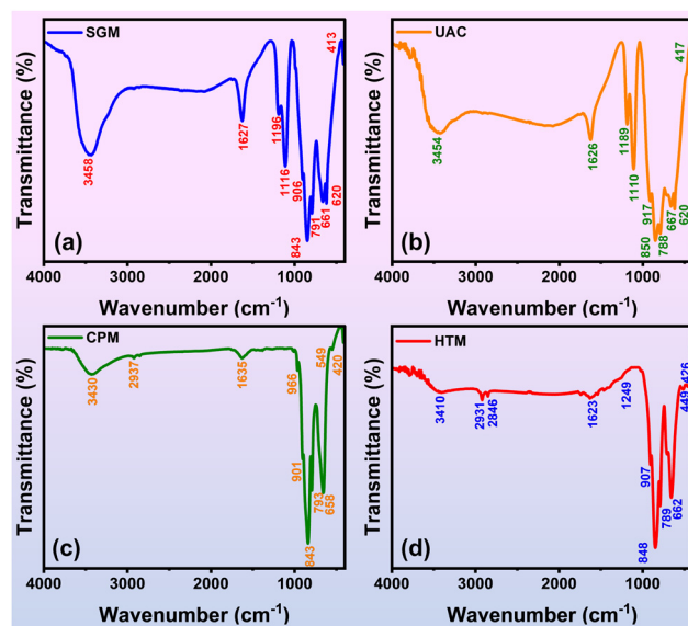
Fig. 2 FTIR spectra of ZnVO nanoposphors synthesized by different methods: (a) SGM, (b) UAC, (c) CPM, and (d) HTM.
