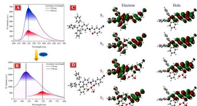
Fig. 27 PL spectra of L 26 compound in THF (A) and 10% water fraction with THF after 12 h standing (B). (C) and (D) Optimized keto structure for S 1 and S 2 state; Reproduced from ref. 121 with permission from Elsevier, copyright 2021.
