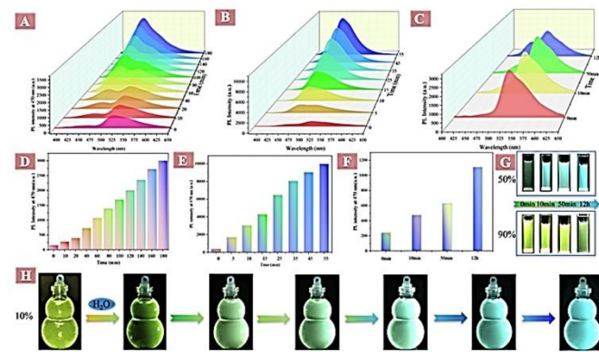
Fig. 12 Changes in fluorescence spectra and intensity of L26 in THF/H 2 O at 470 nm in THF/H 2 O mixtures with different water fractions as 10% (A, D), 50% (B, E), respectively. (G) Changes in emission images of L26 with time 50% and 90% sample. (H) The emission images change of L26 ( 10^{-4} M) in 10% THF/H 2 O mixtures with different time intervals at excitation wavelength 370 nm, excitation wavelength at 370 nm UV; Reproduced from ref. 121 with permission from Elsevier, copyright 2021.
