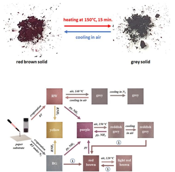
Fig. 20 Thermo and vapochromic behaviour shown by paper substrate containing ML 19 complex; Reproduced from ref. 130 with permission from ACS, copyright 2024.
