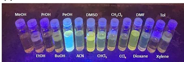
Fig. 13 Fluorescence images of Schiff base ( L 30 ) in different solvents: a) Normal light (no emission), b) upon UV radiation (emission wavelength, \lambda_{\text{em}}=366\text{nm} ) at room temperature; Reproduced from ref. 123 with permission from Elsevier, copyright 2024.
