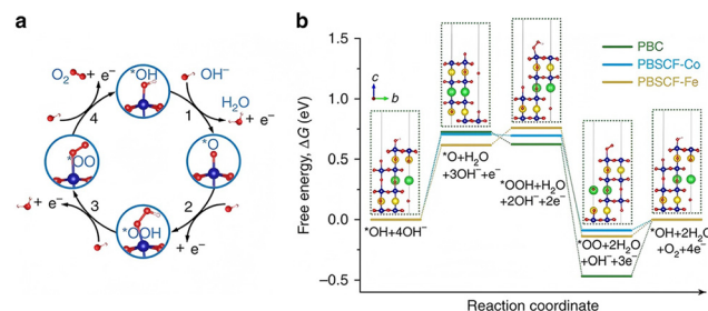
Fig. 26 DFT calculation for the OER mechanism. (a) Illustration of the four electron-proton step mechanism of the OER in alkaline electrolyte. (b) The computed Gibbs free energy changes for the whole system for the OER at \eta = 0 \text{ V/298.15 K} on a \text{PrBaCo}_2\text{O}_{5+\delta} (PBC)/ \text{PrBa}_{0.5}\text{Sr}_{0.5}\text{Fe}_{0.5}\text{O}_{5+\delta} (PBSCF) surface; the B-sites in PBC (Co) and PBSCF (Co/Fe) are treated as the catalytically active centers, all adsorbates are bonded to these redox centers; insets are atomic structures of PBC slabs with adsorbates. In all schematics, each deep blue ball is Co or Fe, fluorescent yellow ball is Pr, green ball is Ba or Sr, red ball is O and light pink ball is H. 101 Copyright 2017, Springer Nature.
