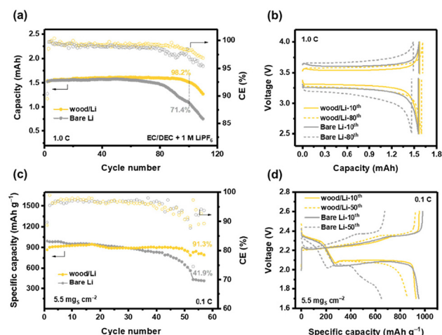
Fig. 5 Electrochemical performances of Li|LFP full cells: (a) long-term cycling performances at 1.0 C and (b) charging-discharging curves at the 10 th and the 80 th cycle, respectively. Electrochemical performances of Li|S full cells with high sulfur areal loading, (c) long-term cycling performances and (d) charging-discharging curves at the 10 th and the 50 th cycle, respectively.
