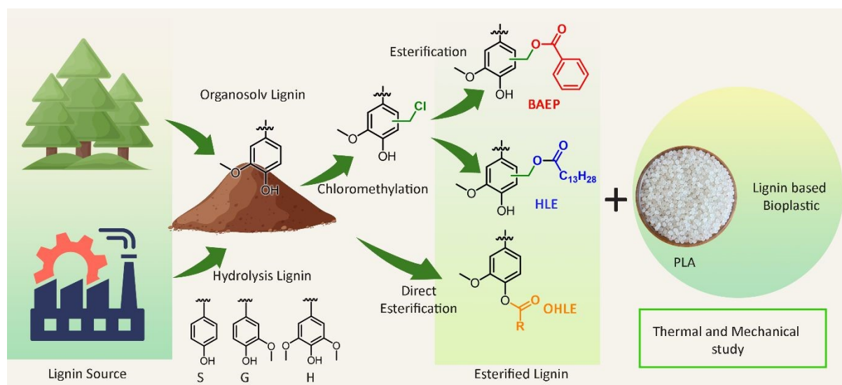
Figure 1. Esterification of organosolv pine lignin and hydrolysis lignin in three different schemes and their compatibility study with PLA.
