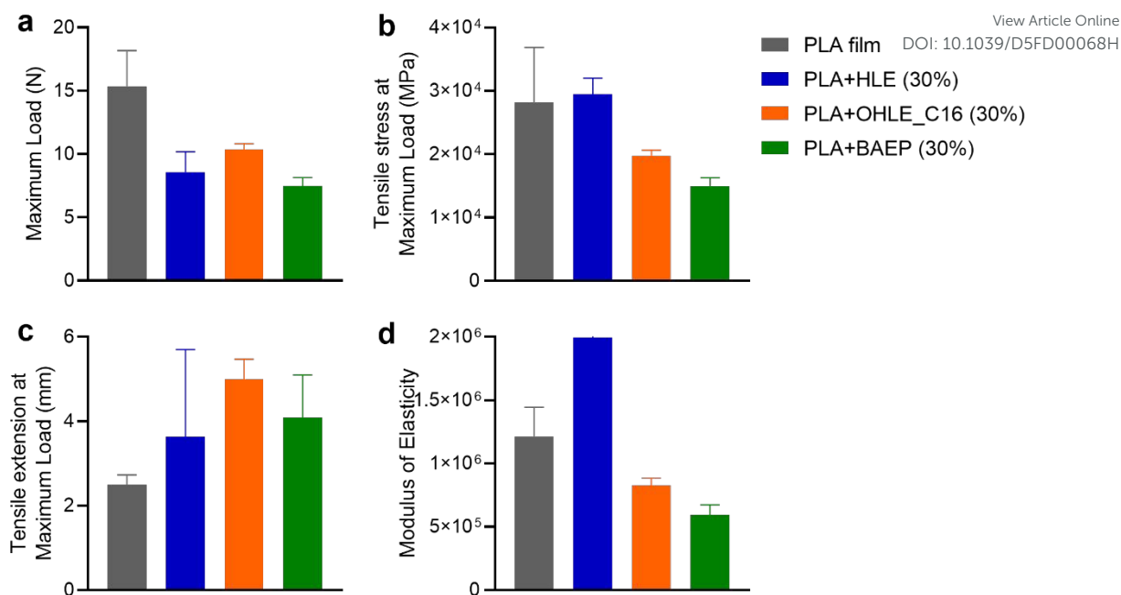
Figure 5. (a) Maximum load, (b) tensile stress at maximum load, (c) tensile extension at maximum load, (d) Young's modulus of PLA/lignin film.
