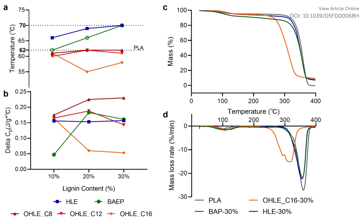
Figure 4. Glass transition temperature (a), delta C_p (b), thermogravimetric (c), and differential thermogravimetric (d) studies for PLA/lignin film.
