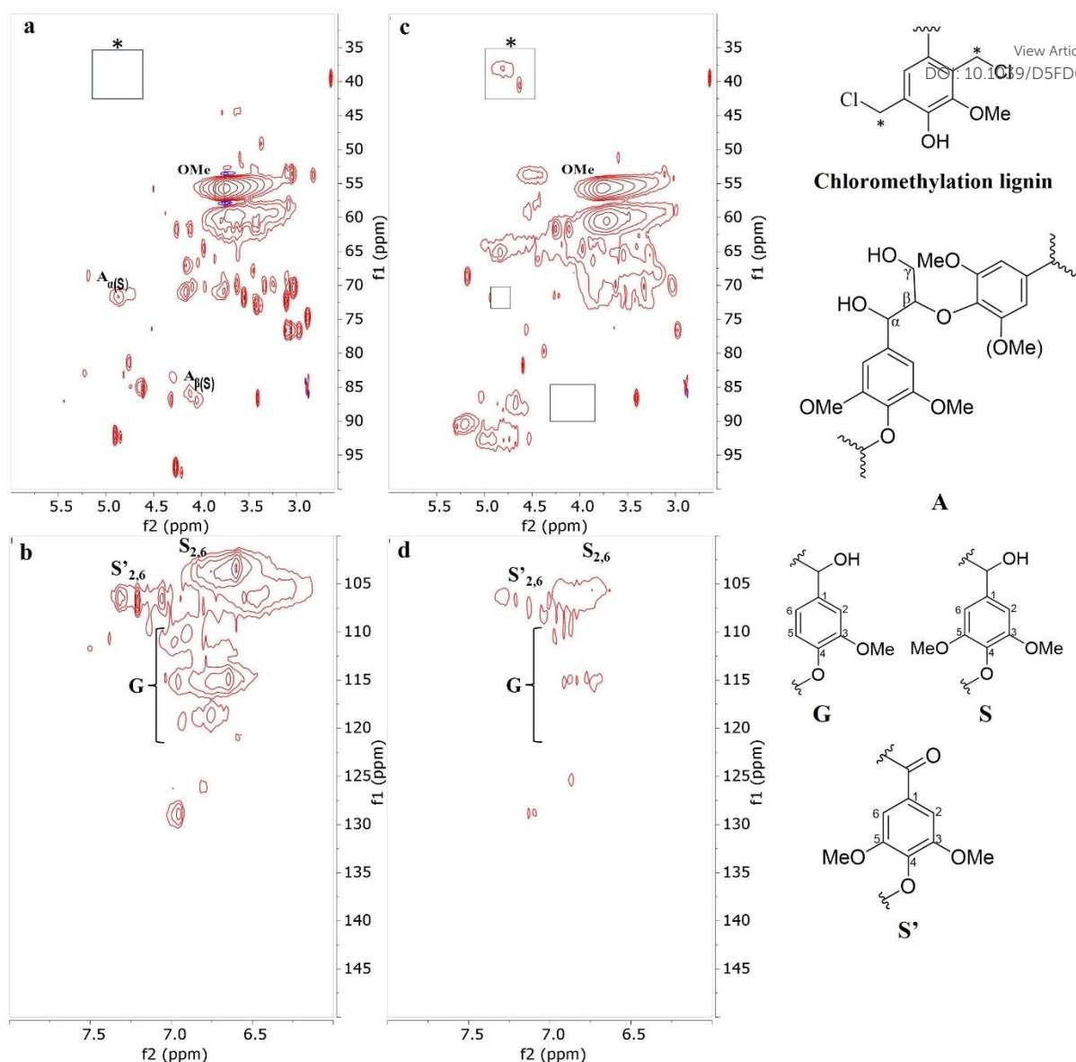
Figure 2. 2D-HSQC of hydrolysis lignin (a, b), chloromethylation lignin (c, d). Two regions of investigation: oxygenated aliphatic side chain (C/H 100–35/6.0–2.5 ppm) (top), aromatic/unsaturated region (C/H 150–100/8.0–6.0 ppm) (bottom). The lignin's subunits are shown on the right side.
