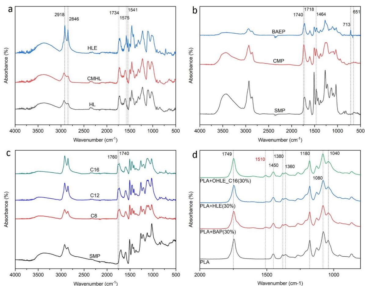
Figure 3. FT-IR measurements for hydrolysis lignin esters (HLE) (a), lignin benzoic acid ester (BAEP)(b), direct esterified lignin (OHLE)(c) derivatives, and PLA/lignin ester films (d).
