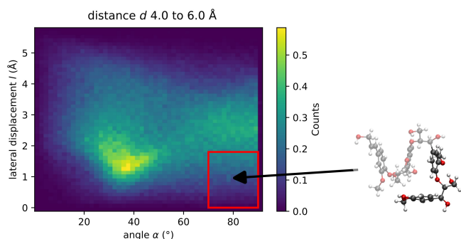
Fig. 5 Left: 2D plot of all angles \alpha and lateral displacements l recorded for rings with the distance d defined as for T-shaped \pi-\pi -stacking. The red square indicates cutoff-values suggested for \alpha and l . Right: Snapshot showing an exemplary conformation of a tetramer that meets the criteria of a T-shaped \pi-\pi -stacking arrangement.
