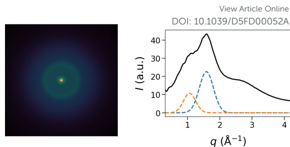
Fig. 7 Simulated WAXS: 2D scattering (left) and 1D integrated peak at relevant q -values including two fitted Gaussian peaks in the same way as previous experiments (right).
