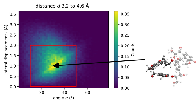
Fig. 4 Left: 2D plot of all angles \alpha and lateral displacements l recorded for rings with the distance d defined as for sandwich-type \pi-\pi -stacking. The red square indicates cutoff-values suggested for \alpha and l . Right: Snapshot showing an exemplary conformation of a tetramer that meets the criteria of a sandwich-shaped \pi-\pi -stacking arrangement.
