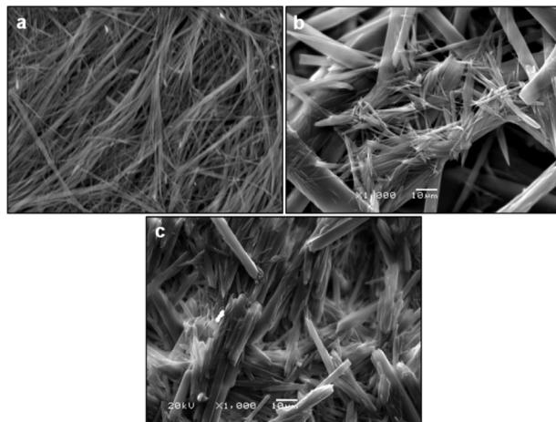
Fig. 5 SEM images of (a) Phe (303 mM), (b) Phe/NH 2 -Phe (1 : 2) and (c) NH 2 -Phe (606 mM) dried hydrogels. The hair-like fibres of Phe had an average width of 1.1 μm (ranging between 0.4 and 1.7 μm), whereas the average width of the needle-like fibres of NH 2 -Phe was 25.3 μm (ranging between 2.6 and 47.9 μm).
