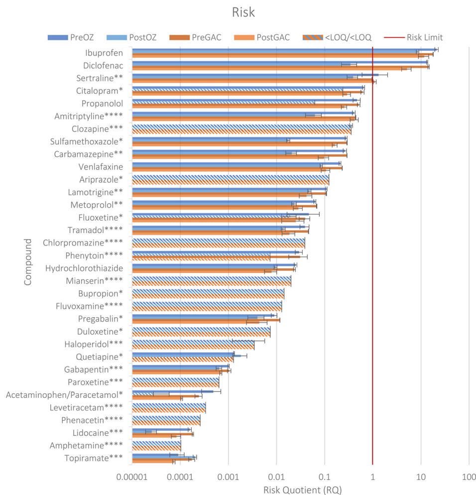
Fig. 2 Risk quotients for all 33 compounds in the study, for all 4 samples. The red line indicates where a risk is seen (i.e. RQ > 1) and the error bars indicate the standard deviation. Striped bars indicate that the risk assessment was based on the LOD or LOQ. Asterisks next to the names indicate the assessment factor used by the NORMAN database. * = 10, ** = 50, *** = 100, **** = 1000 (QSARS only), no asterisk indicates no assessment factor present.
