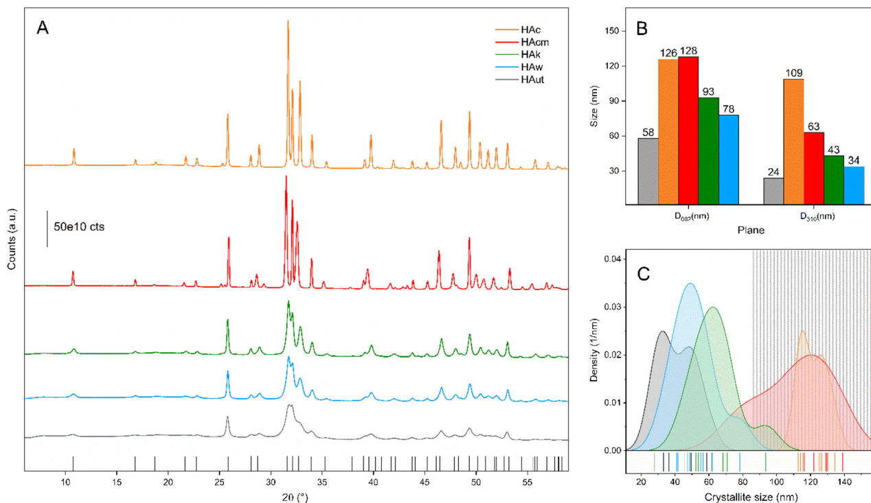
Fig. 5 A) XRD patterns of HA recovered from bovine bones. Vertical black lines below the diffraction patterns represent peak positions of carbonated-hydroxyapatite JCPDS card 969003552. B) Crystallite size dimensions along the [002] and [310] directions. C) Crystallite size distribution plotted employing kernel density. The colored lines below the curves represent individual crystallite size, calculated using the Scherrer equation. The color coding in legend A corresponds to the color used in B and C.
