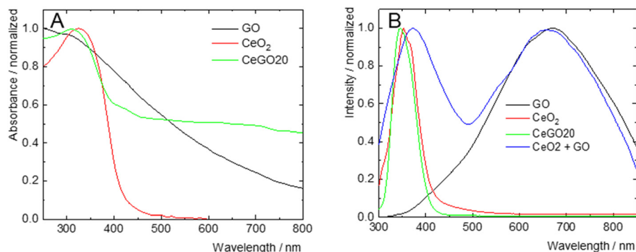
Fig. 4 (A) Normalized absorption spectra of water dispersions of GO, CeO 2 , and CeGO20. (B) Normalized luminescence spectra of water dispersions of GO, CeO 2 , CeGO20, and the physical mixture of CeO 2 and GO, excitation at 250 nm.
