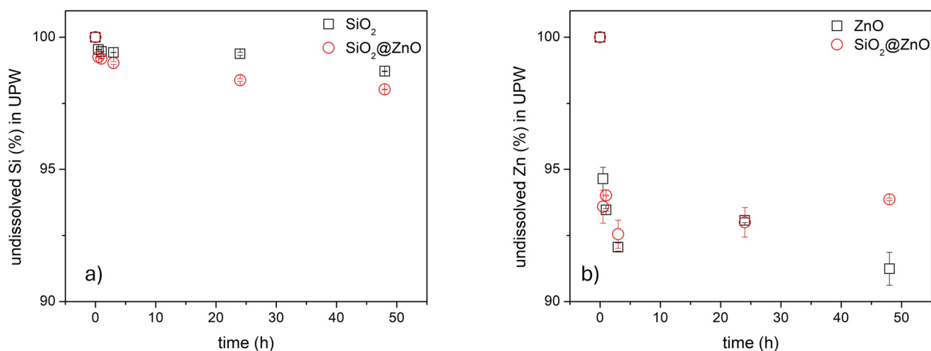
Fig. 7 Dissolution of Si and Zn from both individual and MCNM. a) Si% from SiO 2 NM and SiO 2 @ZnO MCNM. b) Zn% from ZnO NM and SiO 2 @ZnO MCNM.
