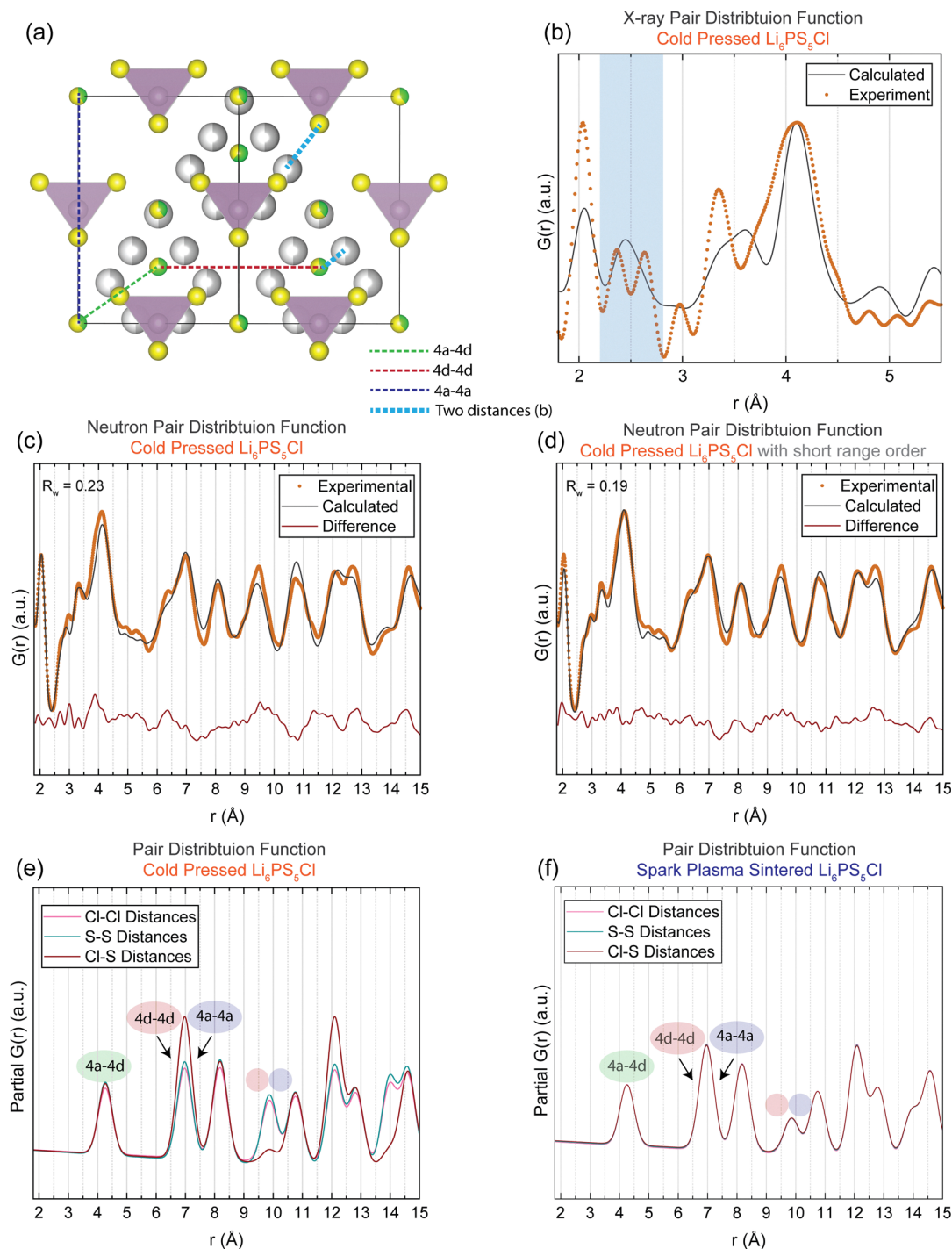
Fig. 4 Short-range order. (a) The structure of \text{Li}_6\text{PS}_5\text{Cl} with the 4a-4d (green), 4a-4a (blue), and 4d-4d (red) distances is given as dashed lines. \text{Li} is shown in grey, \text{P} in purple, \text{S} in yellow and \text{Cl} in green. (b) A comparison of the PDF predicted from the diffraction refinements and the experimental X-ray PDF. Two distinct \text{Li-S/Cl} distances are observed in the experimental data (highlighted in the cyan band), whilst the diffraction simulated PDF predicts a single average distance. These two distances are shown as cyan dashed lines on the structure in (a). (c) The experimental and calculated neutron PDF for the cold-pressed \text{Li}_6\text{PS}_5\text{Cl} , with (d) improvements to the fit observed with the addition of short-range order. All fits, with and without SRO, are given in Fig. S6. (e) The partial PDF for the cold-pressed \text{Li}_6\text{PS}_5\text{Cl} shows preferential 4d-4d and 4a-4a ordering compared to (f) the disordered SPS \text{Li}_6\text{PS}_5\text{Cl} which has no SRO. The presented \text{S-Cl/S} distances are only the 4a/4d environments and do not include the \text{PS}_4 tetrahedra. The blue/red circles highlight the distance of the second 4d-4d and 4a-4a coordination sphere.
