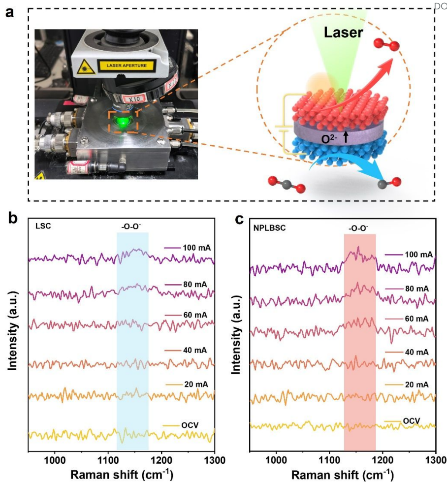
Figure 4. In situ Raman spectroscopy tests. (a) Picture and schematics of the in situ Raman spectroscopy cell. In situ Raman spectra of (b) LSC and (c) NPLBSC at 600 °C, respectively.
