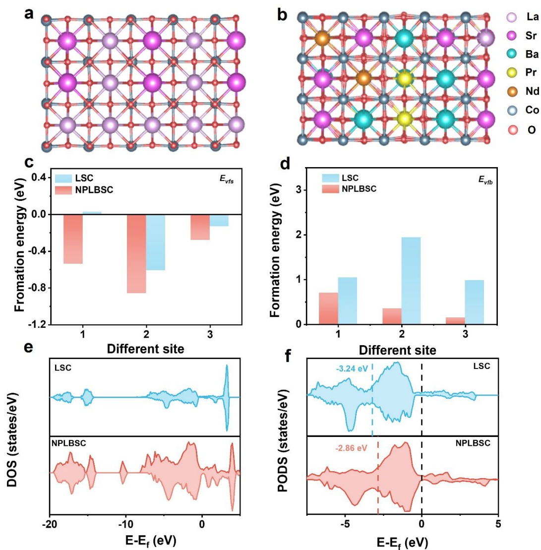
Figure 5. DFT calculation results. The geometric model of (a) LSC perovskite and (b) NPLBSC with random distribution of A site. Diagrams of formation energy of oxygen vacancy (c) on surface and (d) in bulk of the LSC and NPLBSC. (e) Total density of states and (f) partial density of states of the O 2p-band of LSC and NPLBSC and the corresponding band center relative to the Fermi level.
