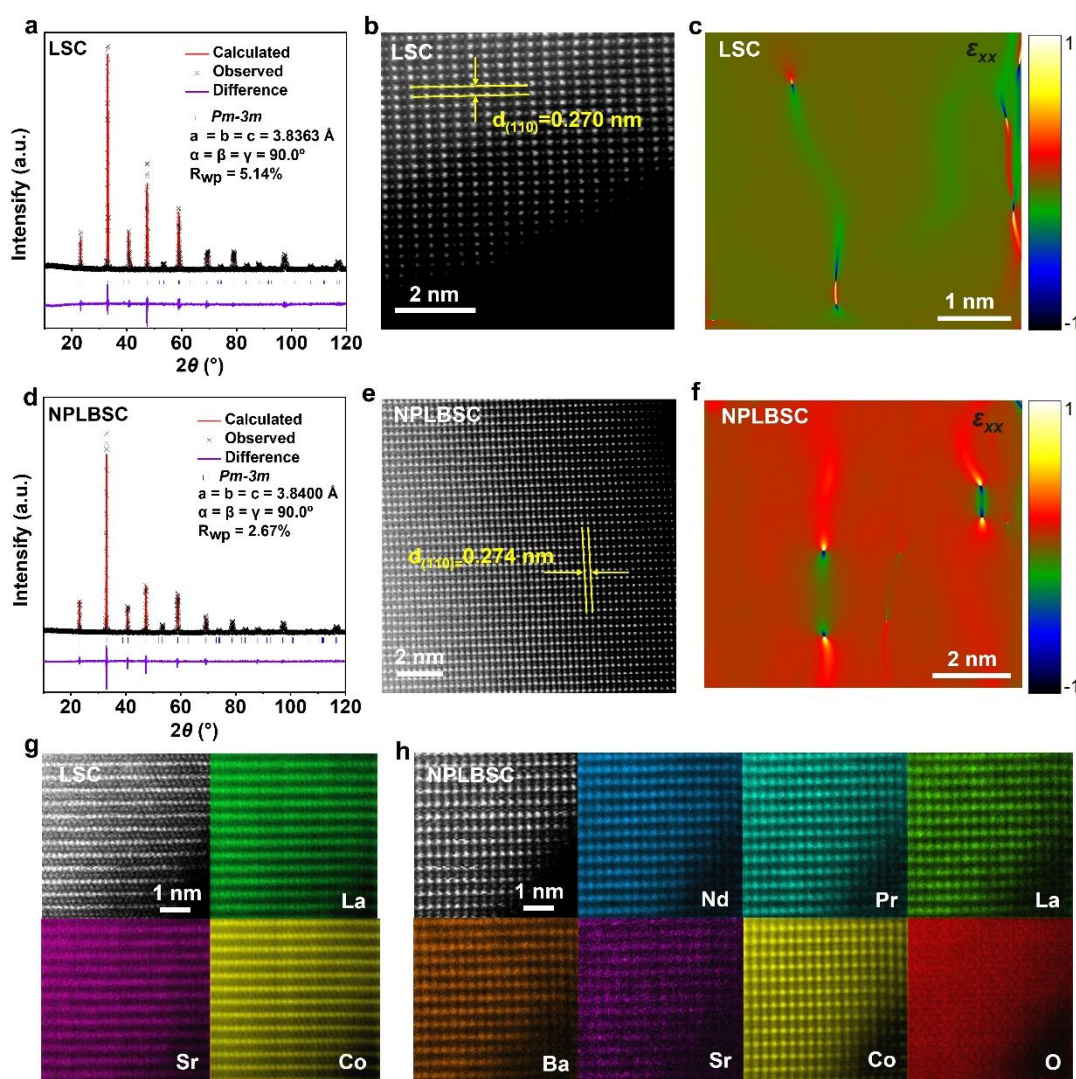
Figure 1. Structural characterizations. Refined XRD patterns of (a) LSC and (d) NPLBSC. HAADF-STEM image of (b) LSC and (e) NPLBSC. Geometric phase analysis (GPA) strain map of \epsilon_{xx} of (c) LSC and (f) NPLBSC. HAADF-STEM elemental maps of (g) LSC and (h) NPLBSC.
