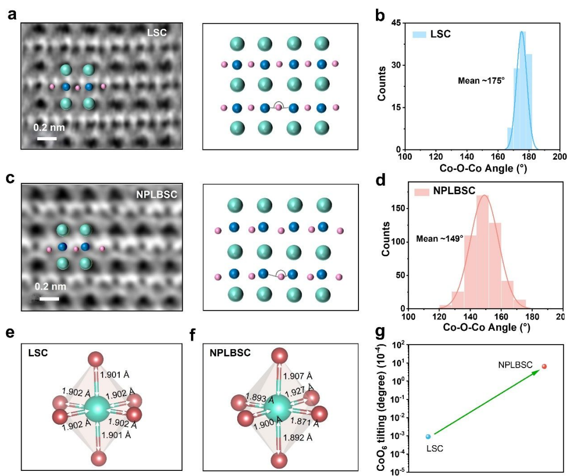
Figure 2. STEM-ABF images of (a) LSC and (c) NPLBSC. Distribution of the Co-O-Co angle in (b) LSC and (d) NPLBSC. Bond structure in \text{CoO}_6 octahedral in (e) LSC and (f) NPLBSC. (g) \text{CoO}_6 octahedral distortion degree ( \Delta ) calculated by the equation \Delta = \frac{1}{6} \sum \left( \frac{R_i - R_{av}}{R_{av}} \right)^2 (where R_{av} is the average bond length, and R_i is the individual bond length of Co-O in \text{CoO}_6 octahedral).
