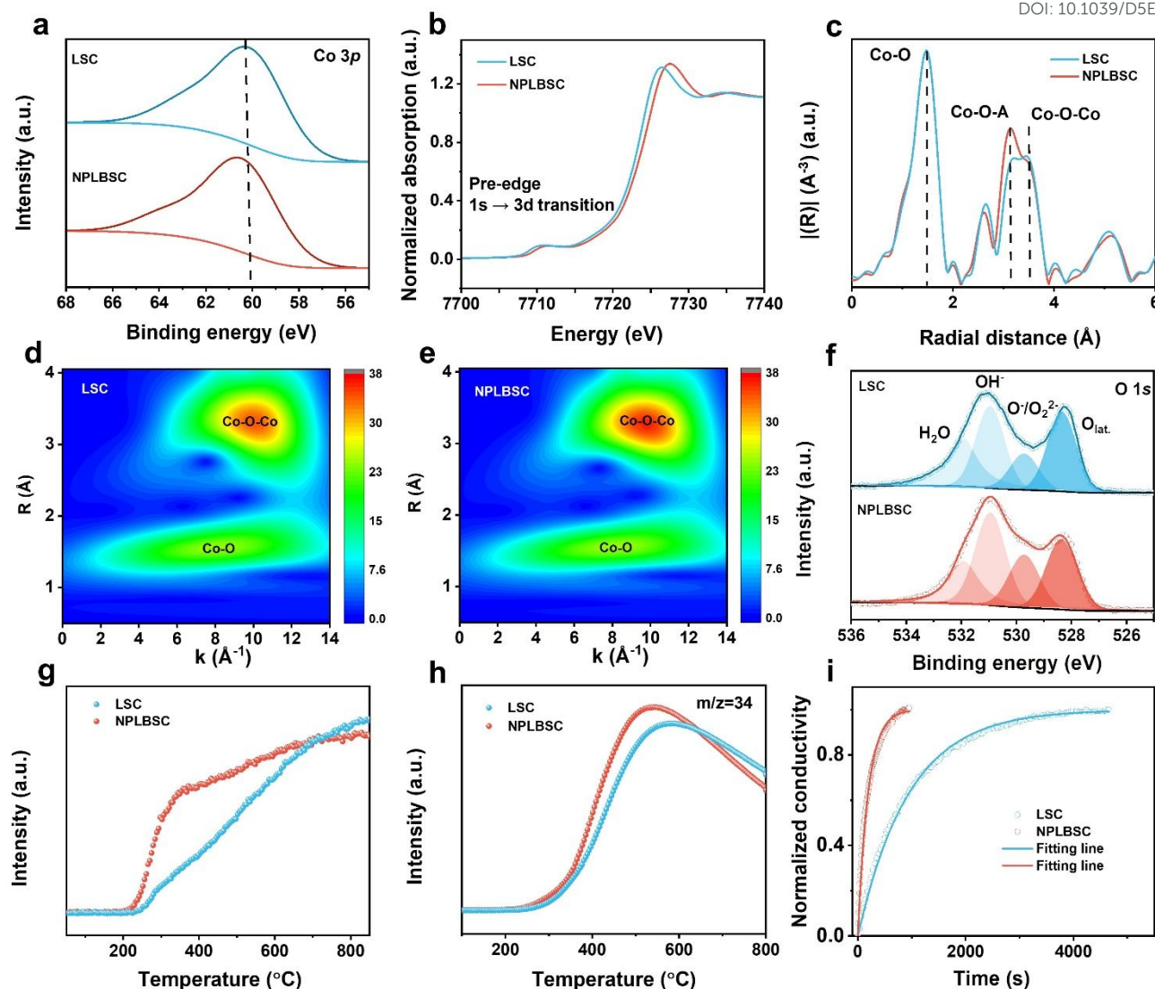
Figure 3. Physicochemical properties of LSC and NPLBSC. (a) XPS spectra of Co 3p. (b) XANES at room temperature. (c) Extended X-ray absorption fine structure spectra (EXAFS) at room temperature. (d) LSC and (e) NPLBSC at room temperature. (f) XPS spectra of O 1s. (g) O 2 -TPD profiles. (h) Results of 18 O isotope exchange experiment. (i) ECR curves at 800 °C.
