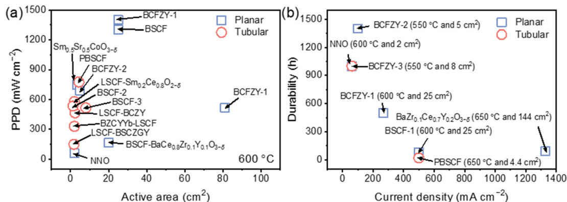
Fig. 15 Large-area P-SOCs: (a) PPDs at 600\text{ }^\circ\text{C} and (b) durability (data detailed in Table 2).
