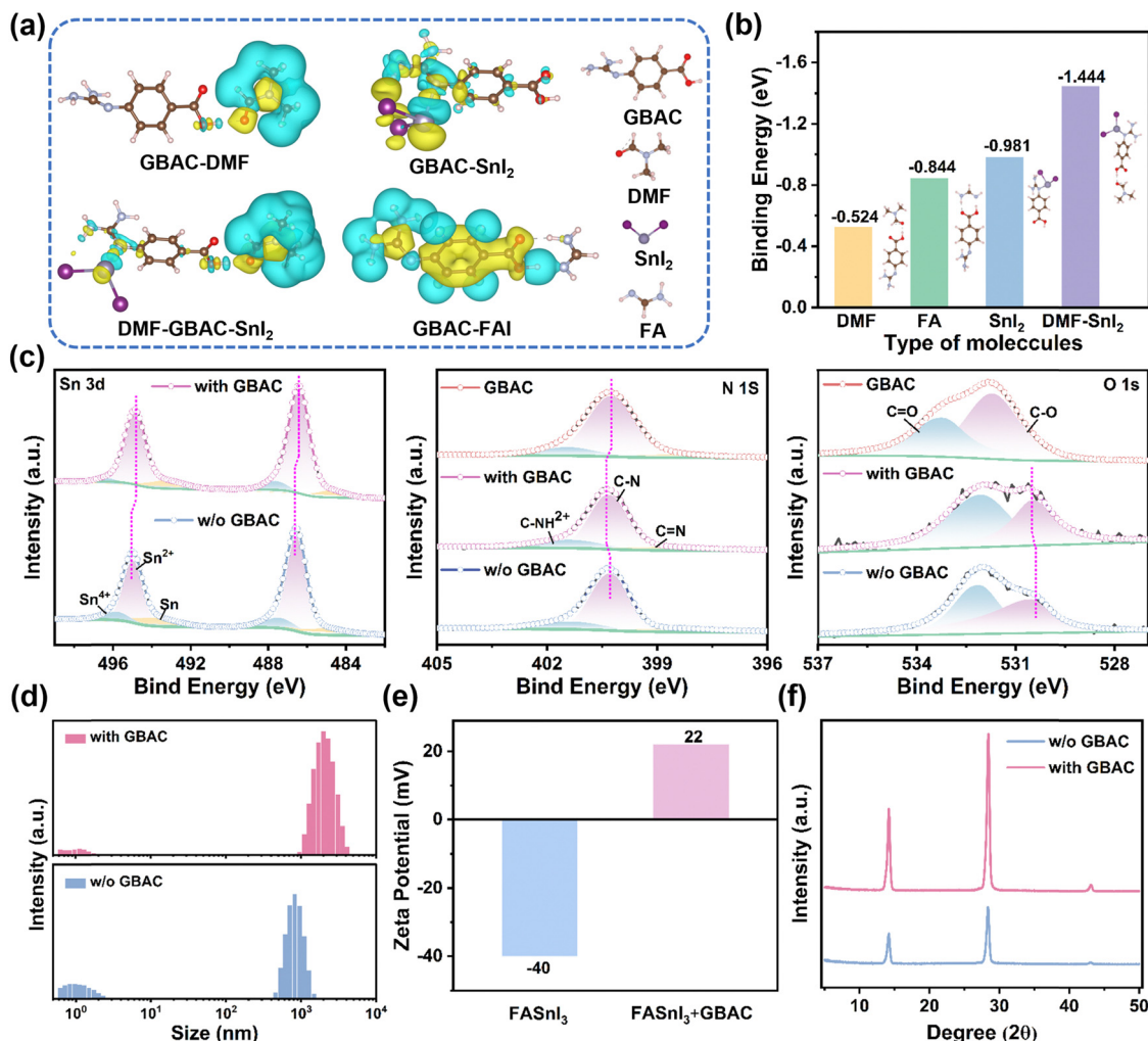
Fig. 3 (a) Distributions of the charge density from DFT and (b) binding energies of DMF, FAI, \text{SnI}_2 , and DMF- \text{SnI}_2 with GBAC, respectively. (c) XPS spectra of Sn, N, and O for films without and with GBAC. (d) Average cluster size and (e) zeta potentials of perovskite precursor solutions without and with GBAC. (f) XRD patterns for tin perovskite films without and with GBAC.
