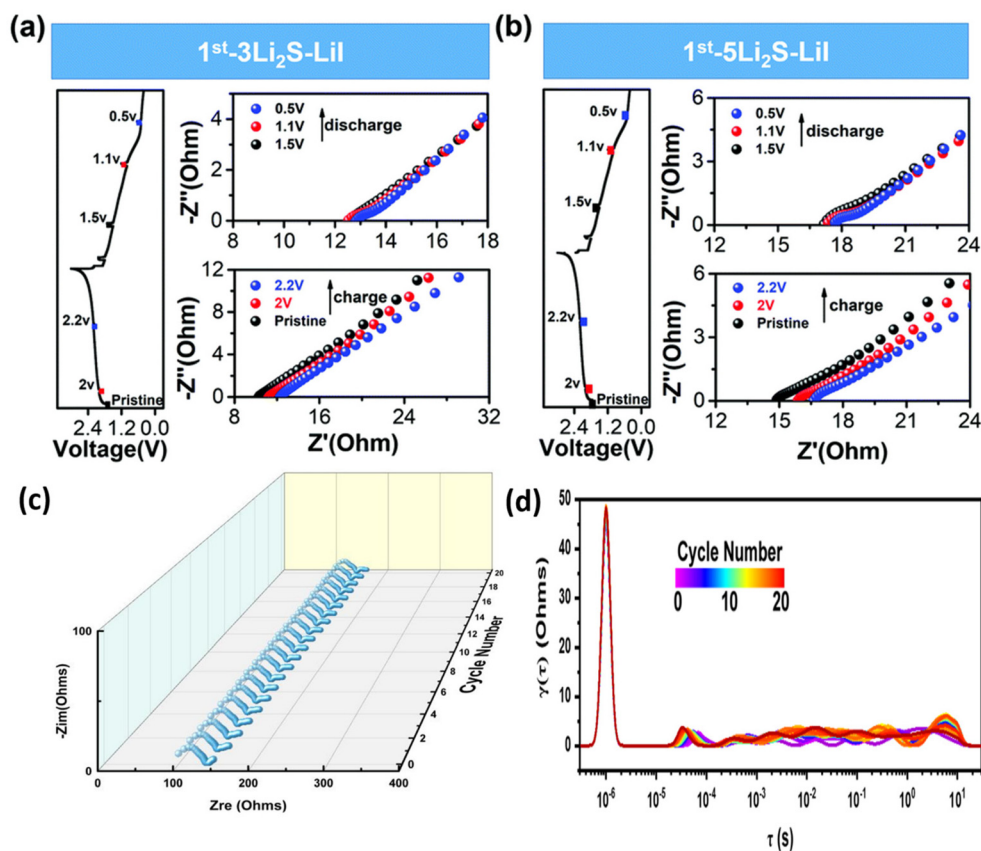
Fig. 24 In situ EIS measurements. In situ EIS performed on \text{Li}_{5.5}\text{PS}_{4.5}\text{Cl}_{1.5} -based ASSLBs, utilizing cathode mixtures of 3\text{Li}_2\text{S-LiL} (a) and 5\text{Li}_2\text{S-LiL} (b) during the first cycle at a CD of 0.13\text{ mA cm}^{-2} , within a voltage range of 0.4 to 3 V vs. Li-In at ambient temperature. 331 (c) In situ EIS of Li|LPS-LGPS-LPS|Li cells operated at 0.1\text{ mA cm}^{-2} and 0.1\text{ mA h cm}^{-2} . (d) DRT results from the in situ EIS of Li|LPS-LGPS-LPS|Li cells operated at 0.1\text{ mA cm}^{-2} and 0.1\text{ mA h cm}^{-2} . 320
