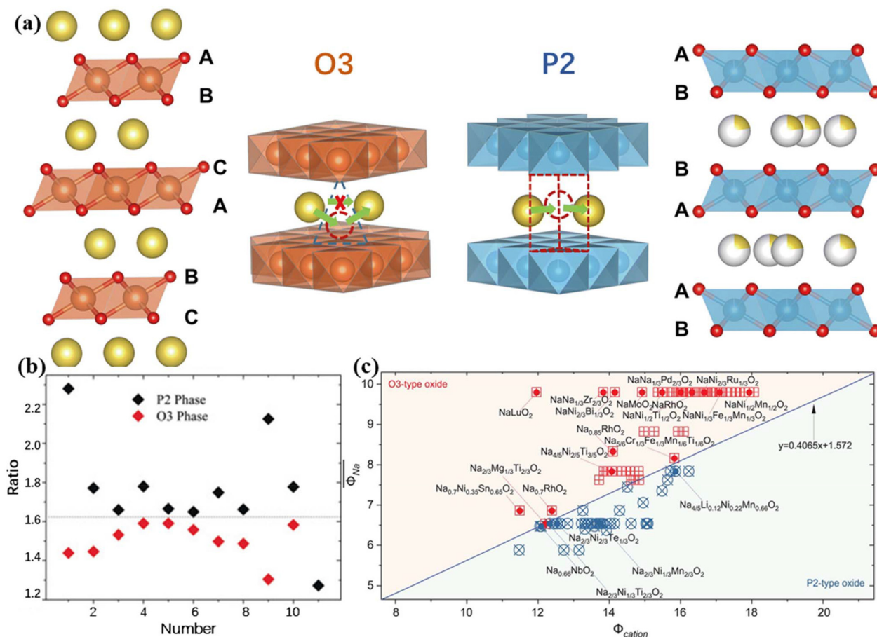
Fig. 2 Crystal structures of O3 and P2 phases and predictive methodologies for their identification. (a) Crystalline structure of layered oxide cathode materials and the \text{Na}^+ migration path. 57 Copyright 2024, Royal Society of Chemistry. (b) The ratio of the interlayer distance between the alkali metal layer d_{(\text{O}-\text{Na}-\text{O})} and the transition metal layer d_{(\text{O}-\text{TM}-\text{O})} . 58 Copyright 2018, Wiley-VCH GmbH. (c) Various sodium based LTMOS with the O3 and P2 structures, which show clear tendency toward each structure depending on the sodium ionic potential and the overall cationic potential. 59 Copyright 2020, The American Association for the Advancement of Science.
