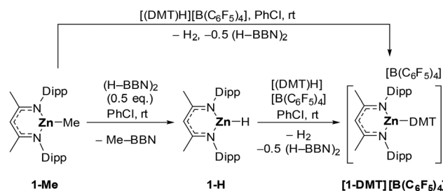
Fig. 5 Formation of [1\text{-DMT}]^+ via two routes starting from 1-Me : direct protonolysis with [(\text{DMT})\text{H}][\text{B}(\text{C}_6\text{F}_5)_4] (top) or initial reaction with (\text{H-BBN})_2 (0.5 eq.) forming 1-H followed by subsequent reaction with the ammonium salt.
