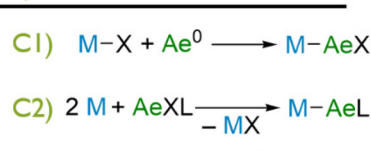
Fig. 1 Synthetic methodologies used to prepared complexes with Ae–M bonds.
