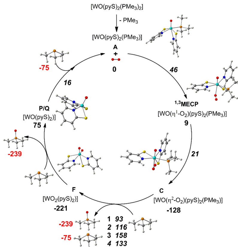
Fig. 5 Calculated catalytic cycle for aerobic oxidation of \text{PMe}_3 catalyzed by tungsten(IV) [\text{WO}(\text{PyS})_2(\text{PMe}_3)_2] (A) (1, 2, 3, 4 refer to the four mechanisms fully described in Fig. 3, S5, S7 and S9 in the SI). (Energies in \text{kJ mol}^{-1} , \Delta G^\ddagger bold, \Delta G^\ddagger bold italic).
