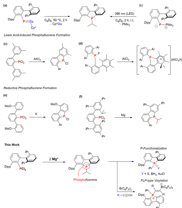
Scheme 1 (a) Thermal phosphinidene release from a phosphagallene, (b) photochemical PMe 3 release from Dipp TerP(PMe 3 ); (c) and (d) Lewis acid induced phosphafluorene formation in terphenyl-substituted halo-phosphanes; (e) and (f) reductive approaches towards phosphafluorenes from dichlorophosphanes (e and f); and summary of this work.
