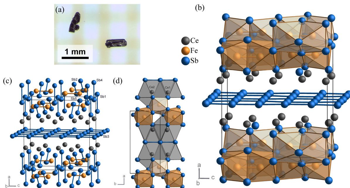
Fig. 1 (a) Flux-grown \text{CeFeSb}_3 crystals. (b) Crystal structure of \text{CeFeSb}_3 approximately along the [010] direction with \text{FeSb}_6 octahedra and \text{Sb}(3) plane. (c) Fe–Fe and shortest Sb–Sb distances shown in a ball-and-stick representation; see text for details. (d) Crystal structure along the [001] direction, revealing the two crystallographically inequivalent Ce sites.
