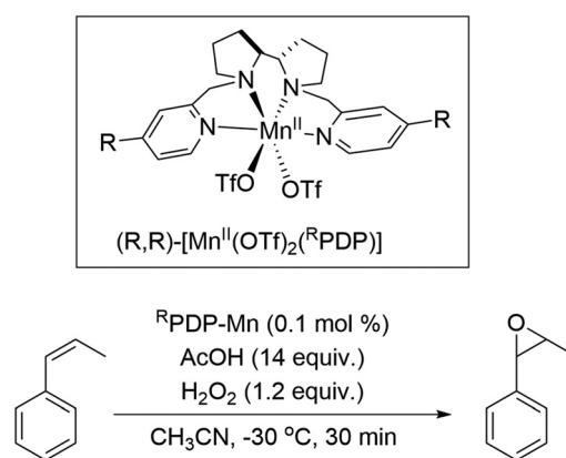
Fig. 2 Manganese ( (R,R)\text{-[Mn}(\text{OTf})_2(\text{R}^{\text{PDP}})] ) catalysed epoxidation of cis - \beta -methylstyrene with \text{H}_2\text{O}_2 . 26
