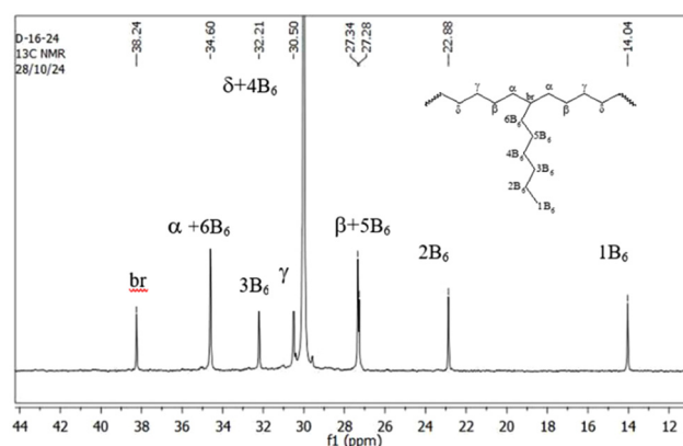
Fig. 3 ^{13}\text{C}\{^1\text{H}\} NMR spectrum of the copolymer produced by VO(acac) 2 (4-phenylpyridine)/EtAlCl 2 (D-16-24).
