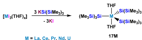
Scheme 3 Synthetic access to a number of trisilylated ate-complexes 17M .
