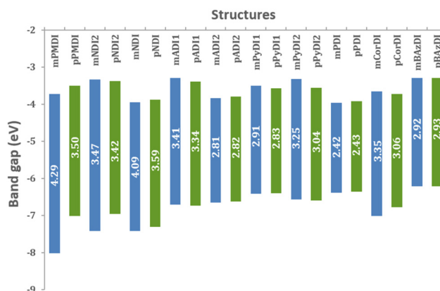
Fig. 3 Band gap energy of rylene diimides.
