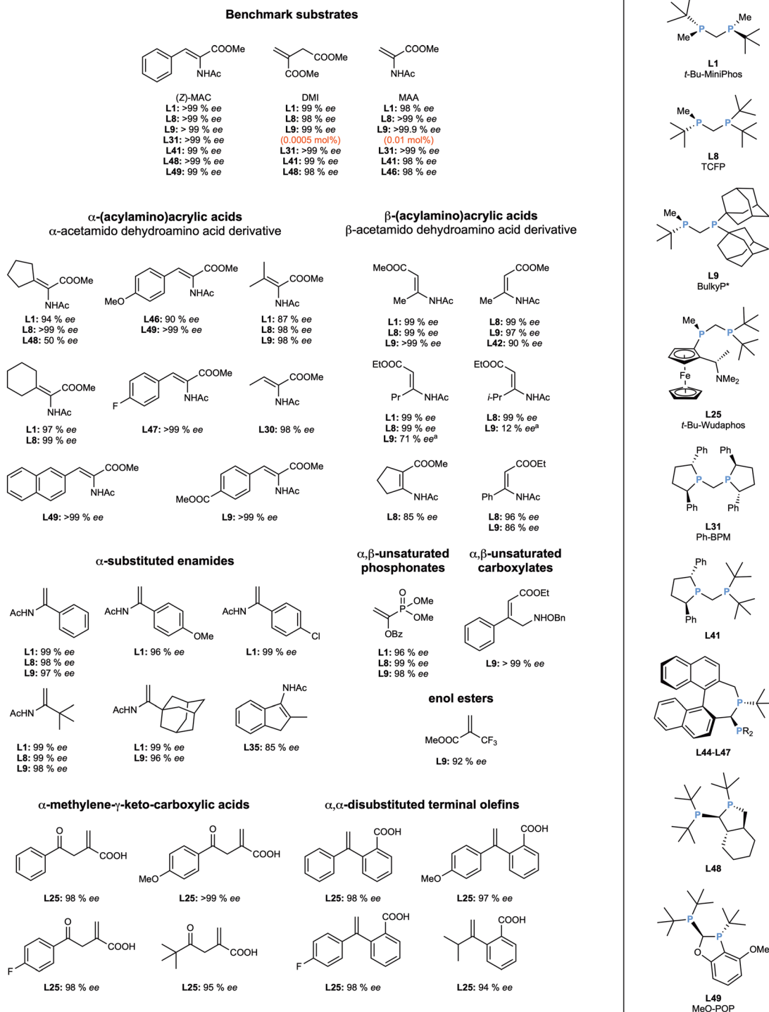
Fig. 5 Selected substrates used in Rh-catalysed enantioselective hydrogenation with PCP ligands and their corresponding enantioselectivities. a (Z)-isomer.
